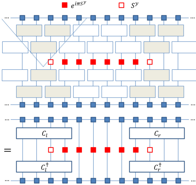
FIG. 2. (Color online) The expectation value \langle \psi | C^\dagger Q C | \psi \rangle . The horizontal lines attached with small blue squares represent \langle \psi | (bra) or |\psi\rangle (ket), and the short rectangles are the 2-local unitaries in C . The (white) unitaries outside the causal cones (dotted lines) of S^y (small open red squares) can be removed, as they are symmetric. Then we merge the (gray) symmetric local quantum gates inside each causal cone into one symmetric quantum gate (long rectangle) of sublinear support.
