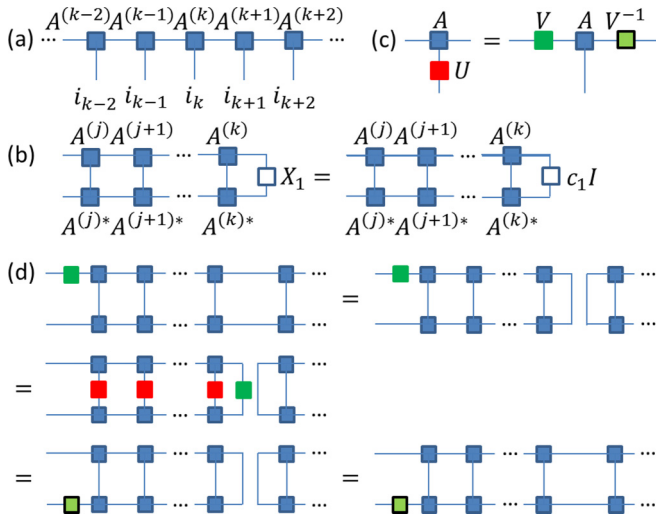
FIG. 3. (Color online) (a) Graphical representation of MPS (B4) [37]. Each square represents a tensor A^{(k)} with two bond indices (horizontal lines) and one physical index (vertical line). The bond indices are contracted sequentially with periodic boundary conditions (not shown). (b) The condition (B6) for short-range correlated MPS. The graphical equation is approximate up to error e^{-\Omega(k-j)} , which can be neglected in the thermodynamic limit N \rightarrow +\infty if k-j = \Theta(N) . (c) Graphical representation of (B8). The site labels are not shown. (d) is a consequence of (b) and (c). Note that a prefactor of the second, third, and fourth tensor networks is not shown.
