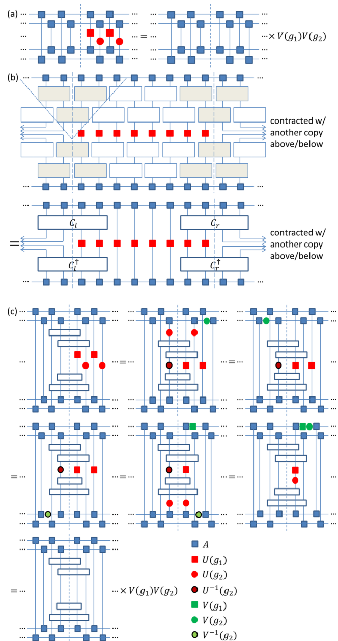
FIG. 5. (Color online) (a) The domain wall (dashed line) that contributes the local phase factor V(g_1)V(g_2) [9]. (b) The short rectangles are the local unitaries in C . The (white) unitaries outside the causal cones (dotted lines) of the domain walls can be removed, as they are symmetric. Then we merge the (gray) symmetric local quantum gates inside each causal cone into one symmetric quantum gate (long rectangle) of sublinear support. (c) Graphical proof of the invariance of the local phase factor for the domain wall in (a) under symmetric local quantum circuits of sublinear depth.
