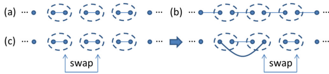
FIG. 1. (Color online) The renormalization group (RG) fixed-point states [15,22] in the (a) trivial and (b) nontrivial fermionic (Majorana chain) or SPT (e.g., Haldane chain) phases. For states in fermionic phases, each dot represents a Majorana mode and connected pairs form fermionic modes which are vacant or occupied. For states in SPT phases, each dot carries a projective representation of the symmetry group and connected pairs form symmetric singlets. (c) The states in (a) and (b) can be exactly mapped to each other with a linear-depth 2-local quantum circuit composed of SWAP gates.
