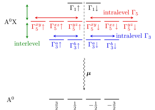
FIG. 2. (Color online) Full energy level diagram for A^0X and A^0 system. The spin of the electron is denoted by \uparrow, \downarrow . Intralevel and interlevel relaxation cause a decay of the polarization visibility [Fig. 3(b)]. Electron spin flips are not allowed, as depicted schematically by the dashed line. The crystal fields that split \Gamma_3 and \Gamma_5 lead to \hat{x}, \hat{y}, \hat{z} oriented along the crystallographic axes.
