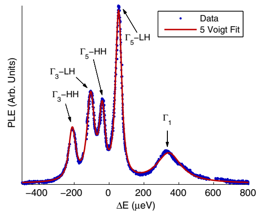
FIG. 9. (Color online) Photoluminescence excitation spectroscopy of A^0 X . The method of mounting the sample introduces strain, which splits the heavy-hole and light-hole ground states. A linear offset due to donor acceptor pair emission was subtracted for clarity. The curve was fit to a sum of five Voigt functions.
