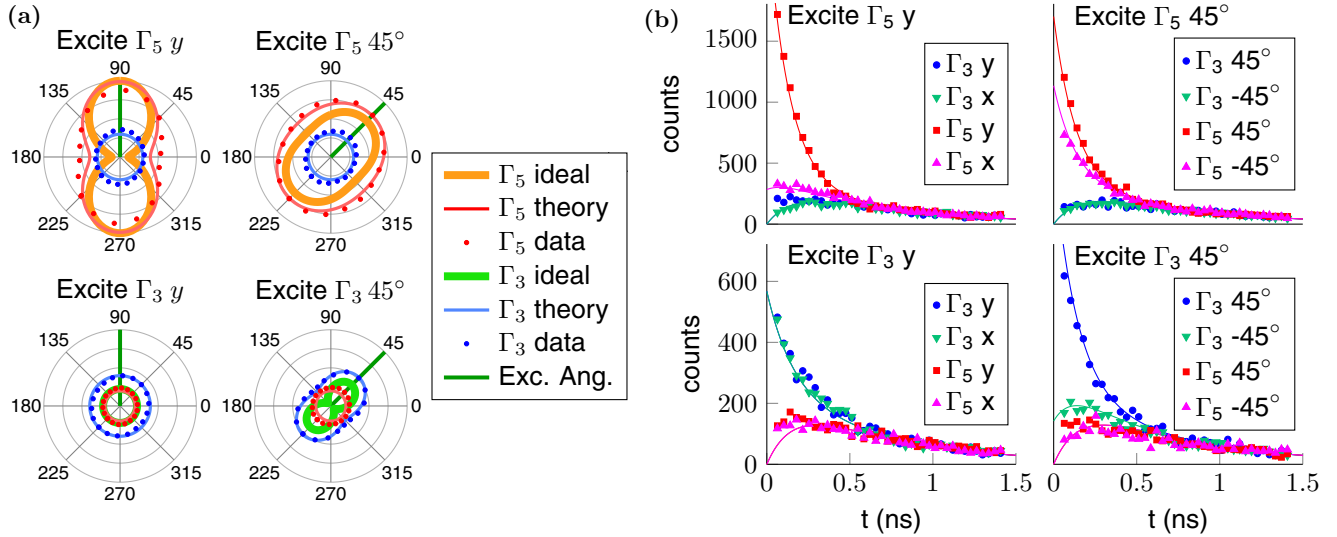
FIG. 3. (Color online) (a) Dependence of light emitted from \Gamma_3 and \Gamma_5 on incident and collected polarization for A^0X \rightarrow A^0 relaxation in resonant CW excitation. The dark green line shows the angle of excitation polarization, with horizontal \hat{x} corresponding to [100] . The polar plots show the PL emitted at the corresponding collection polarization angle. The ideal theory curves depict the polarization dependence in the absence of excited state relaxation. The theory curves give the angular PL dependence expected from the density matrix model fit to the time-resolved data [Fig. 3(b)]. The data are PL collected from the |A^0X, \Gamma_n\rangle \rightarrow |A^0, 2s\rangle transition while exciting the \Gamma_3 or \Gamma_5 line at \hat{x} or \frac{1}{\sqrt{2}}(\hat{x} - \hat{y}) = -45^\circ polarizations (Fig. 1). All the data are normalized using the same constant. The normalization between the ideal curves and the theory curves is arbitrary. T = 2.3 K. (b) The \Gamma_3 and \Gamma_5 PL as a function of time for polarizations x \propto [100] , y \propto [010] , 45^\circ \propto [110] , and -45^\circ \propto [1\bar{1}0] after an excitation pulse at t = 0 . The lines are a simultaneous fit of the density matrix model to the 16 observed time dependent PL curves. Best fit parameters are given in the text.
