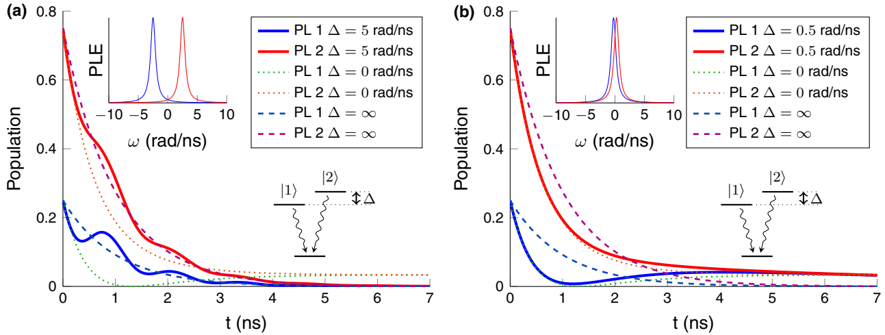
FIG. 6. (Color online) Time dependence of excited state population depending on detuning between two excited states that can interfere. \tau = 1 ns. For a detuning \Delta much larger than the spontaneous emission rate 1/\tau , the population of the two excited states decay independently. When \Delta = 0 , the lifetimes are modified by interference of the two recombination pathways, and the system progresses towards a dark state. The lifetimes of states in the absence of interference are 1 ns for both transitions. The initial wave function is |\psi\rangle = \frac{1}{2}|1\rangle + \frac{\sqrt{3}}{2}|2\rangle . (a) At intermediate \Delta = 5 rad/ns, some interference is seen in the emission, oscillating around the behavior expected for two independent subsystems. (b) When the transitions are nearly resonant, the emission follows the behavior for degenerate excited states.
