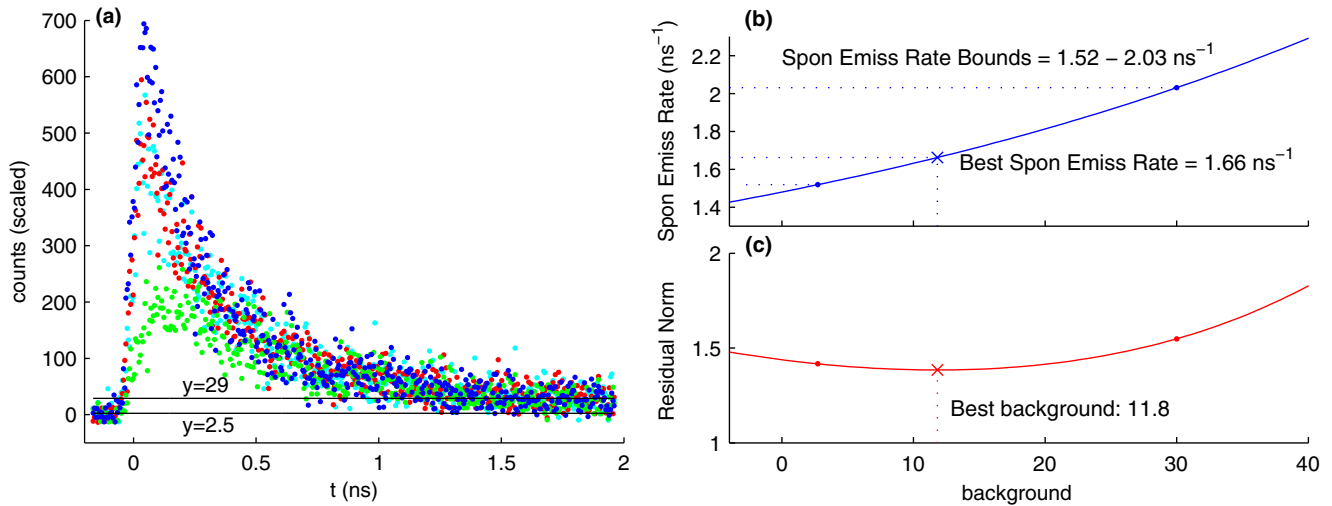
FIG. 7. (Color online) (a) Raw data before binning used for time-resolved experiment. Before the pulse arrives, the mean background level is 2.5 \pm 0.6 counts. At the end of the trace at 2 ns, the mean level is 29 \pm 6 , which is somewhat higher than the theory would predict. (b) and (c) Best fit spontaneous emission rate as a function of background level in the model. The best fit background value lies in between the limits chosen by inspection in (a). These limits are used to find the uncertainty in the spontaneous emission rate due to the background level.
