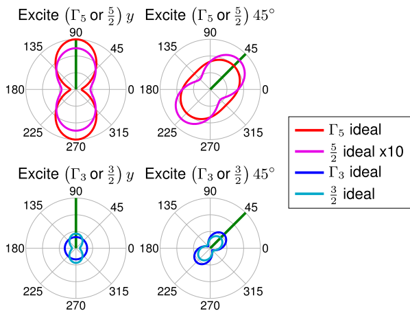
FIG. 8. (Color online) Comparison of polarization dependence of photoluminescence for the JJCS and CFS. Qualitatively different behavior is observed when exciting \Gamma_3 y or \frac{3}{2} y . This difference can be used to determine the validity of the CFS for describing A^0 X .
