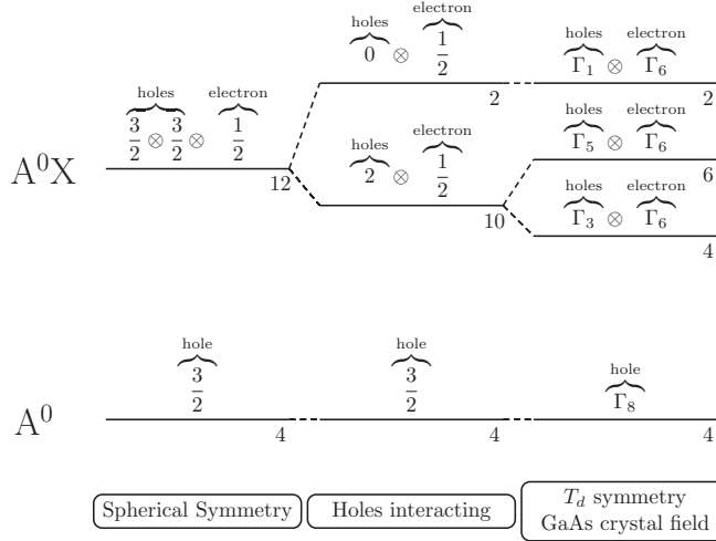
FIG. 5. Hole-hole coupling causes the j = 2 states to be split from the j = 0 states. Crystal fields breaking spherical symmetry and split \Gamma_3 and \Gamma_5 . The degeneracy of the level is shown in the bottom right corner.
