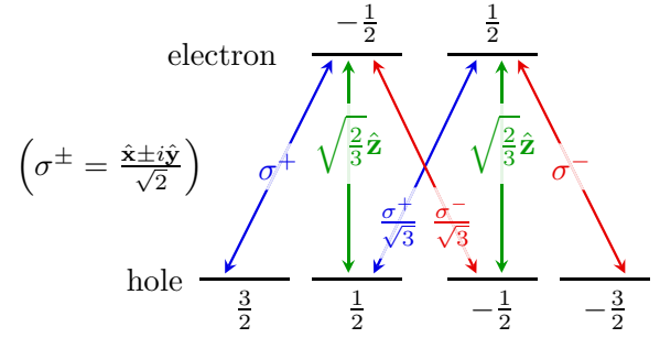
FIG. 4. (Color online) Dipole matrix elements for exciton recombination [1]. The labeled arrows show the polarization of light emitted upon recombination of the corresponding electron-hole pair.
