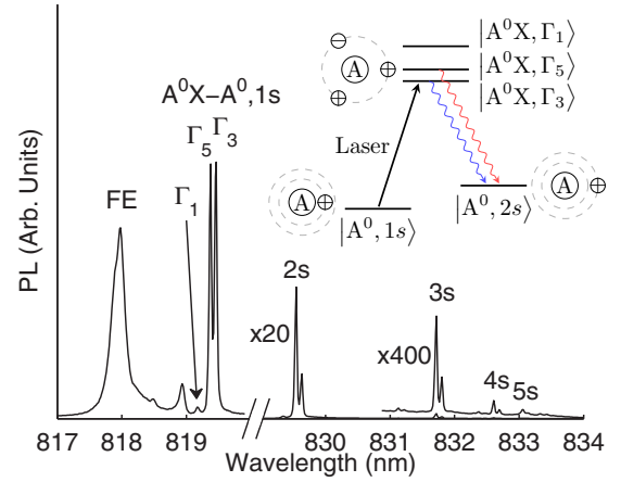
FIG. 1. (Color online) PL spectrum of |A^0X\rangle \rightarrow |A^0, ns\rangle and free exciton (FE) transitions using above band and resonant excitation. The A^0X \Gamma_3 - \Gamma_5 splitting is clearly resolved. The spectrum left of the cut was taken using above band excitation at 815 nm. The spectrum right of the cut used resonant excitation of |A^0, 1s\rangle \rightarrow |A^0X, \Gamma_5\rangle . Because of spin relaxation between A^0X states, the different excitation conditions result in different \Gamma_3 to \Gamma_5 intensity ratios left and right of the cut. The inset shows an energy level diagram and cartoon of the A^0 - A^0X system. T = 2.3 K.
