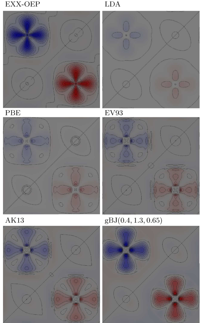
FIG. 10. (Color online) Two-dimensional plots of the difference between spin-up and spin-down exchange potentials ( v_x^\uparrow - v_x^\downarrow ) in a (001) plane of antiferromagnetic NiO. The contour lines start at -2 \text{ Ry} (blue color) and end at 2 \text{ Ry} (red color) with an interval of 0.235 \text{ Ry} . The Ni atom with a full spin-up 3d shell is at the left upper corner.
