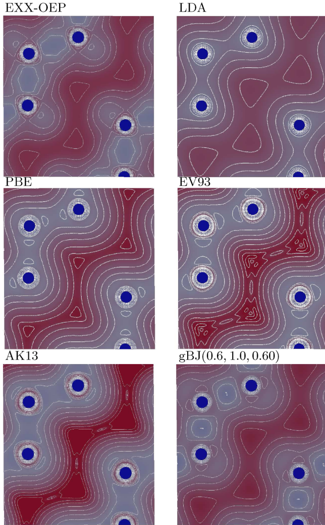
FIG. 6. (Color online) Two-dimensional plots of exchange potentials v_x in a (110) plane of C. The potentials were shifted such that \int_{\text{cell}} v_x(\mathbf{r})d^3r = 0 . The contour lines start at -2 Ry (blue color) and end at 1 Ry (red color) with an interval of 0.2 Ry.
