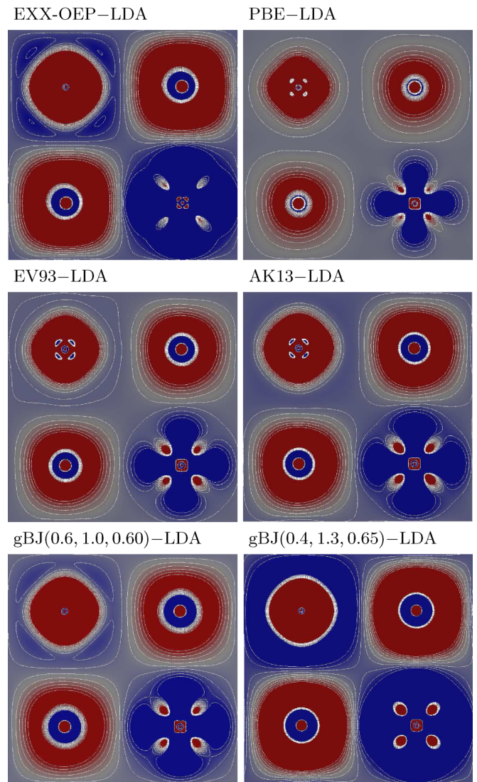
FIG. 12. (Color online) Spin-up electron density \rho_{\uparrow} obtained with different exchange potentials minus \rho_{\uparrow}^{\text{LDA}} plotted in a (001) plane of antiferromagnetic NiO. The contour lines start at -0.005 electrons/bohr 3 (blue color) and end at 0.005 electrons/bohr 3 (red color) with an interval of 0.001 electrons/bohr 3 . The Ni atom with a full spin-up 3d shell is at the left upper corner.
