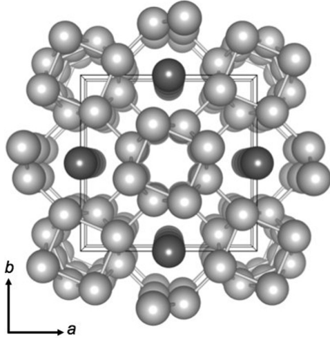
FIG. 1. The composite incommensurate structure of K-IIIa, as viewed down the c axis. The tetragonal 16-atom host component is shown in light gray, and the guest atom chains in dark gray. A unit cell is shown by the solid lines, and the crystallographic axes are labeled.
