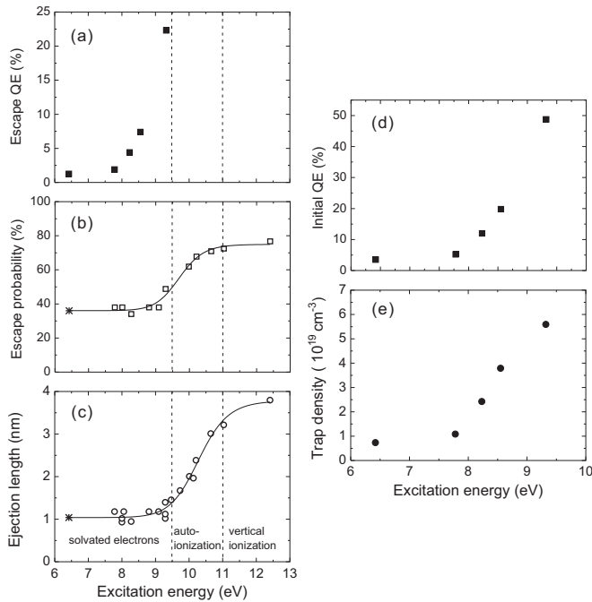
FIG. 1. Literature data on solvated electron generation and ionization pathways in liquid water. (a) Energy dependence of quantum efficiency QE_{\text{esc}} for the creation of long-lived solvated electrons e_{\text{aq}}^-(\text{esc}) that have escaped geminate recombination [32]. (b) Probability P_{\text{esc}} for excess electrons to escape recombination [30]. (c) Average ejection length r_{\text{ej}} of the excess electrons [30]. (d) Initial quantum efficiency QE_{\text{ini}} of excess electron formation derived from (a) and (b) by QE_{\text{ini}} = QE_{\text{esc}}/P_{\text{esc}} . (e) Density of preexisting trap sites for solvated electron formation derived from (c) and (d) by \chi_{\text{trap}} = QE_{\text{ini}}/(4/3\pi r_{\text{ej}}^3) . The energy dependence of P_{\text{esc}} and r_{\text{ej}} in (b) and (c) suggests that vertical ionization into the CB dominates for E_{\text{exc}} \geq 11 eV, and autoionization becomes important for E_{\text{exc}} \geq 9.5 eV. For E_{\text{exc}} < 9.3 eV, all excess electrons relax into the solvated state or recombine. Nevertheless, breakdown initiation is possible if e_{\text{aq}}^- absorb further photons that promote them into the CB, as depicted as “upconversion path” in Fig. 2.
