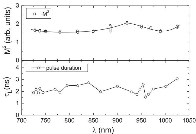
FIG. 5. Wavelength dependence of duration and M^2 values of laser pulses used in the present paper determined for focusing at \text{NA} = 0.9 . The beam quality is optimal around the center wavelength of each of the two optics sets used for the OPO and deteriorates at the borders of each range. Since the M^2 values exhibited little scatter and a clear M^2(\lambda) trend, measurements were performed for only 12 wavelengths, and intermediate values were interpolated. For the pulse duration, no systematic dependence on \lambda is observed.
