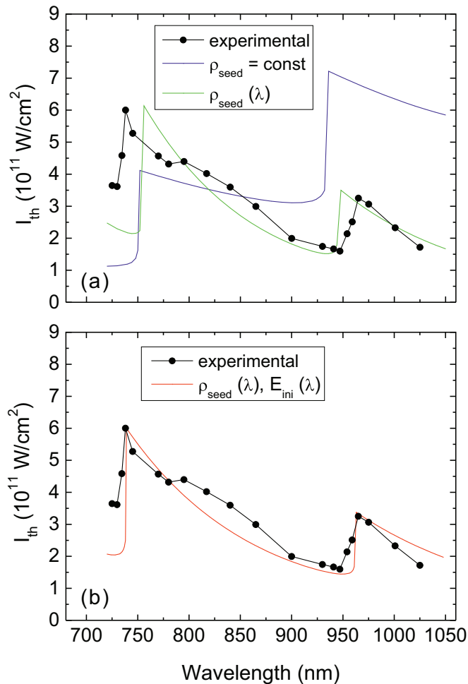
FIG. 8. (Color) Comparison of predictions for I_{\text{th}}(\lambda) based on Eq. (2), with the experimentally determined spectrum (average values from both NAs). Calculations were performed for 2 ns pulse duration. (a) Fits for E_{\text{ini}} = 6.6 \text{ eV} assuming either a constant \rho_{\text{seed}} value of 3.3 \times 10^{14} \text{ cm}^{-3} (blue line) or a wavelength-dependent seed electron density that varies according to \rho_{\text{seed}}(\text{cm}^{-3}) = 10^{A\lambda(\text{nm})+B} (green line). (b) Fit assuming a wavelength-dependent \rho_{\text{seed}} and a linear decrease of E_{\text{ini}} from 6.7 eV at the position of the first peak to 6.43 eV at the second peak (red line; for fit parameters see text).
