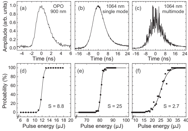
FIG. 4. Pulse shape of a SLM OPO pulse of 900 nm wavelength and 2.3 ns duration (a), compared to single-frequency and longitudinal multimode Nd:YAG laser pulses of 1064 nm wavelength and 11.2 ns duration in (b) and (c), respectively. Below each pulse shape, the corresponding breakdown probability curves are shown in (d)–(f). The threshold sharpness is given by S = E_{th}/\Delta E , with \Delta E being the energy range between 10 and 90% breakdown probability.
