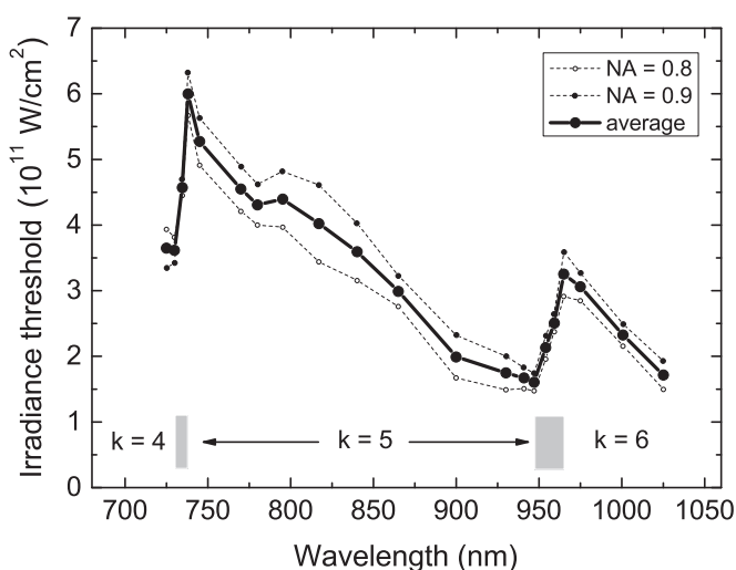
FIG. 6. Wavelength dependence of the threshold for plasma-mediated bubble formation by SLM OPO pulses focused at NA = 0.8 and NA = 0.9 and averaged values. The order of the multiphoton process required to cross the band gap in different regions of the I_{th}(\lambda) spectrum is denoted by k . Transition zones are marked in gray.
