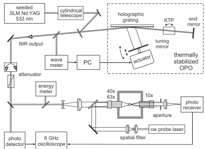
FIG. 3. Setup for the examination of the wavelength dependence of IR ns optical breakdown in water by means of a SLM OPO.
