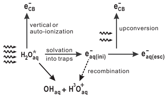
FIG. 2. Ionization and geminate recombination pathways in liquid water, as suggested by the data in Fig. 1. For large excitation energies, ionization can proceed via vertical ionization ( E_{\text{exc}} \geq 11 eV) or autoionization ( E_{\text{exc}} \geq 9.5 eV), while for E_{\text{exc}} < 9.3 eV, ionization is possible only as a two-step process involving solvated electron creation followed by upconversion of e_{\text{aq}}^- into the CB. The latter process competes with geminate recombination.
