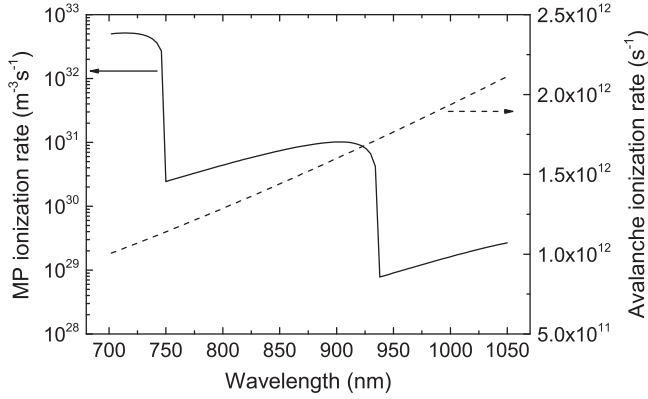
FIG. 7. Wavelength dependence of AI rate (dashed line) and MPI rate (solid line) calculated for E_{\text{gap}} = 9.5 eV and E_{\text{ini}} = 6.6 eV, respectively. The MPI rate is plotted in log scale, while AI rate is in linear scale. All calculations assume an irradiance of 3.5 \times 10^{11} W/cm 2 , which is the average I_{\text{th}} value in the investigated wavelength range.
