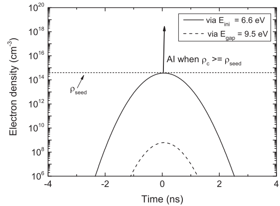
FIG. 9. Temporal evolution of the density of electrons entering the CB via photoionization. The solid line depicts \rho_{\text{ini}}(t) obtained via the initiation channel through multiphoton excitation into the intermediate energy level, E_{\text{ini}} = 6.6 \text{ eV} , followed by immediate upconversion into the CB. The dashed line represents the electron density produced by MPI across the entire band gap, E_{\text{gap}} = 9.5 \text{ eV} , which is almost six orders of magnitude smaller than \rho_{\text{ini}} . Calculation parameters are the same as for Fig. 8(b) at \lambda = 800 \text{ nm} : I_{\text{th}} = 3.76 \times 10^{11} \text{ W/cm}^2 , t_{\text{gem-rec}} = 60 \text{ ps} , and \rho_{\text{seed}} = 3.67 \times 10^{14} \text{ cm}^{-3} . The arrow indicates the time at which the critical seed electron density for AI is reached (45 ps after the peak of the 2 ns laser pulse). Afterwards, the free-electron density rapidly increases to full ionization [4,64].
