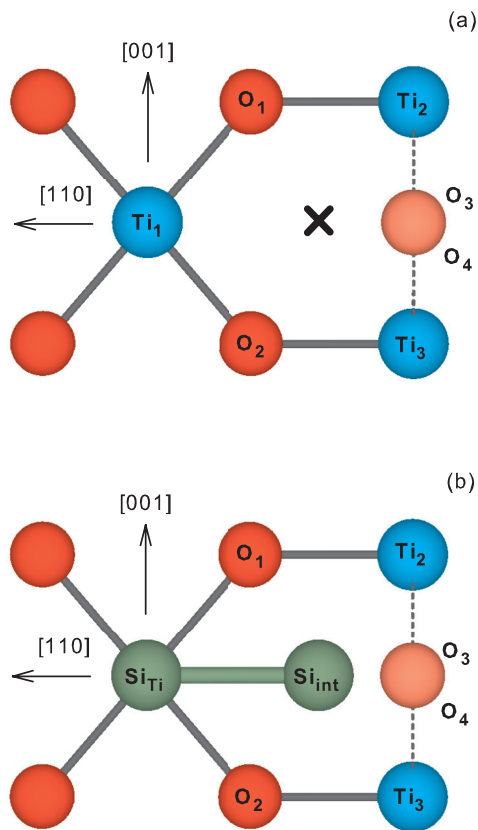
FIG. 7. (Color online) (a) A projection on the [1\bar{1}0] plane of the regular \text{TiO}_2 crystal. Oxygen ions are red, and titanium ions are blue. The oxygen ion labeled \text{O}_3 is in front of the plane, and the oxygen ion labeled \text{O}_4 is behind the plane. A bold \times marks the tetrahedral interstitial position along the [110] direction. (b) Model of the [\text{Si}_{\text{int}} - \text{Si}_{\text{Ti}}]^+ defect.
