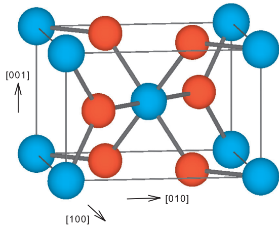
FIG. 1. (Color online) Schematic of the rutile TiO 2 crystal structure, showing one of the two equivalent TiO 6 octahedra and its eight neighboring Ti neighbors.
