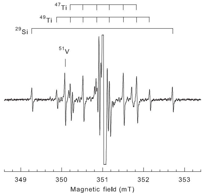
FIG. 2. EPR spectrum of the [Si int – Si Ti ] + defect in an as-grown oxidized rutile TiO 2 crystal. The sample temperature was 40 K, the magnetic field was along the [001] direction, and the microwave frequency was 9.520 GHz. The sample was exposed to 442-nm laser light while acquiring the spectrum.
