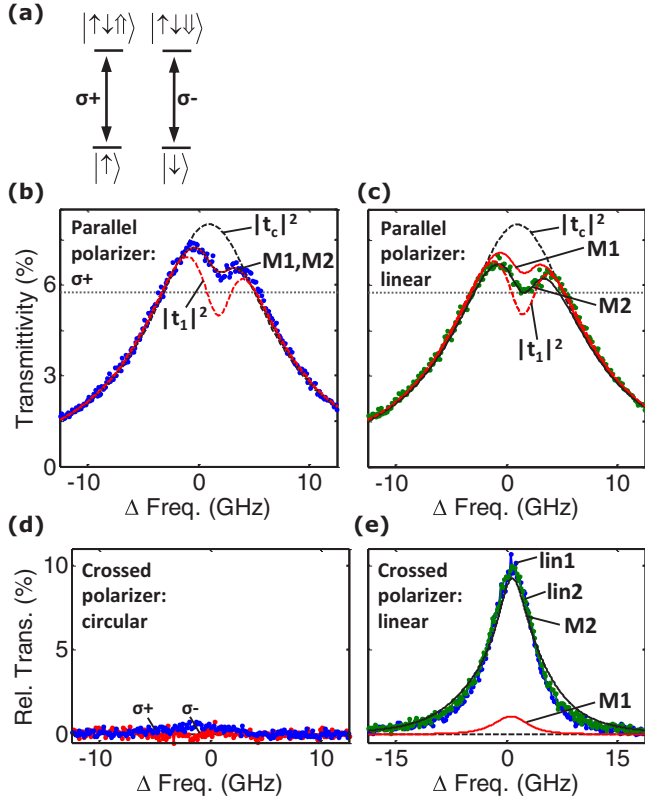
FIG. 4. (Color online) (a) Energy-level diagram of a singly charged QD. Transmission spectra for P_{\text{laser}} = 10 pW are shown for circular and linear polarization, analyzed with a (b) and (c) parallel or (d) and (e) crossed polarizer. The red-black dashed line in (b) is a fit of Eq. (4) (coherent model, M1) to the data, which yields the same result as Eq. (5) (decoherent model, M2). The red (black) solid lines in (c) and (e) predict the experimental data using Eq. (4) [Eq. (5)]. Black (red) dashed curves: empty (coupled) cavity calculations.
