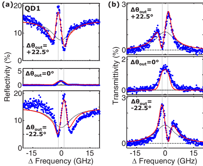
FIG. 3. (Color online) Resonant (a) reflection and (b) transmission spectroscopy with a neutral QD (QD1 in Fig. 2) for \theta_{\text{in}} = 45^\circ and for various \theta_{\text{out}} = \theta_{\text{in}} + 90^\circ + \Delta\theta_{\text{out}} . Blue dots: experimental data. Red lines: predicted curves using Eqs. (1) and (2) and the parameters obtained from the fits in Figs. 2(b) and 2(c). Gray lines: predicted curves corresponding to an empty cavity. Vertical dashed lines mark the two transitions split by the fine-structure interaction.
