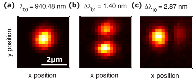
FIG. 5. (Color online) Spatial PL scans of the Hermite-Gaussian modes, where (a) is the fundamental mode \Psi_{00} and (b) and (c) are the first-order \Psi_{10}/\Psi_{01} modes. Light: more PL counts. The labels denote the wavelength \lambda_{00} of the fundamental mode or the wavelength splitting \Delta\lambda_{10/01} = \lambda_{00} - \lambda_{10/01} .
