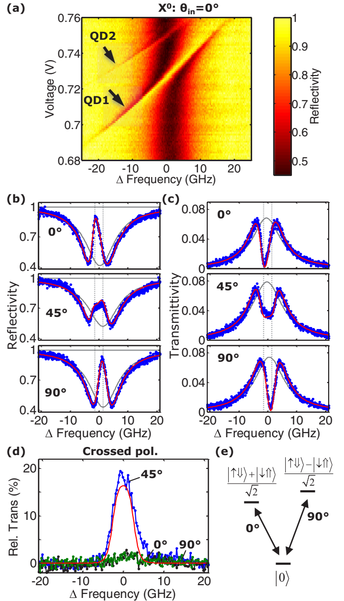
FIG. 2. (Color online) (a) Reflectivity measurement of two neutral QDs as a function of the scanning laser frequency and applied voltage. The incoming polarization \theta_{\text{in}} = 0^\circ , P_{\text{laser}} = 1 pW, and \lambda \approx 940 nm. (b) Reflectivity and (c) transmittivity spectra of QD1 recorded at V = 0.725 V for various incoming linear polarizations. Blue points: experimental data. Red line: fitted curve using Eqs. (1) and (2). Gray curve: empty cavity, calculated from the fits. Vertical dashed lines: frequencies corresponding to the two fine-split transitions. (d) Transmittivity spectra when a crossed polarizer is used with respect to the incoming polarization, relative to the maximum transmittivity of an uncoupled cavity. The red line is calculated using Eqs. (1) and (2) and the parameters obtained from the fits in (b) and (c). (e) Energy-level diagram of the ground-state and lowest-energy excited states of a neutral QD.
