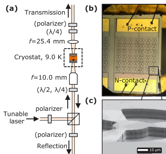
FIG. 1. (Color online) (a) Schematic of the setup. Light is coupled into a microcavity mode, and the reflection and transmission spectra are recorded using single-photon avalanche photodiodes. The elements with names between brackets can be introduced for polarization analysis with either linear or circularly polarized light. \lambda/2 ( \lambda/4 ): half-wave (quarter-wave) plate. (b) Optical microscope image of a sample. (c) Electron micrograph of the cavity region.
