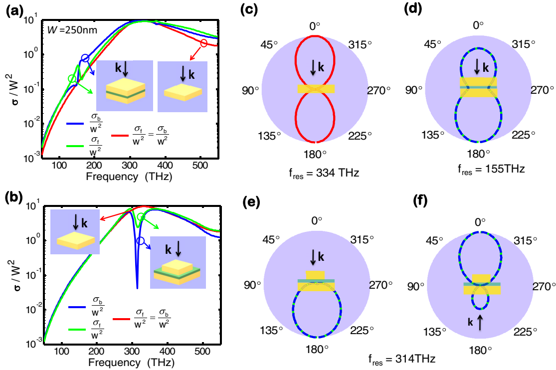
FIG. 4. (Color online) (a) and (b) Comparison between forward and backward frequency dependent normalized radar scattering sections for a single nanopatch (shown in red only since backward and forward radar scatterings are identical), two identical coupled nanopatches, and two nonidentical nanopatches (shown in green and blue) with W_1/W_2 = 0.4 . Illumination occurs as shown in the inset. Electric field patterns of (c) a single nanopatch and (d) two identical coupled nanopatches at resonance. (e) and (f) Corresponding electric field patterns of two nonidentical coupled nanopatches for both backward and forward illumination directions at the resonance frequency, respectively.
