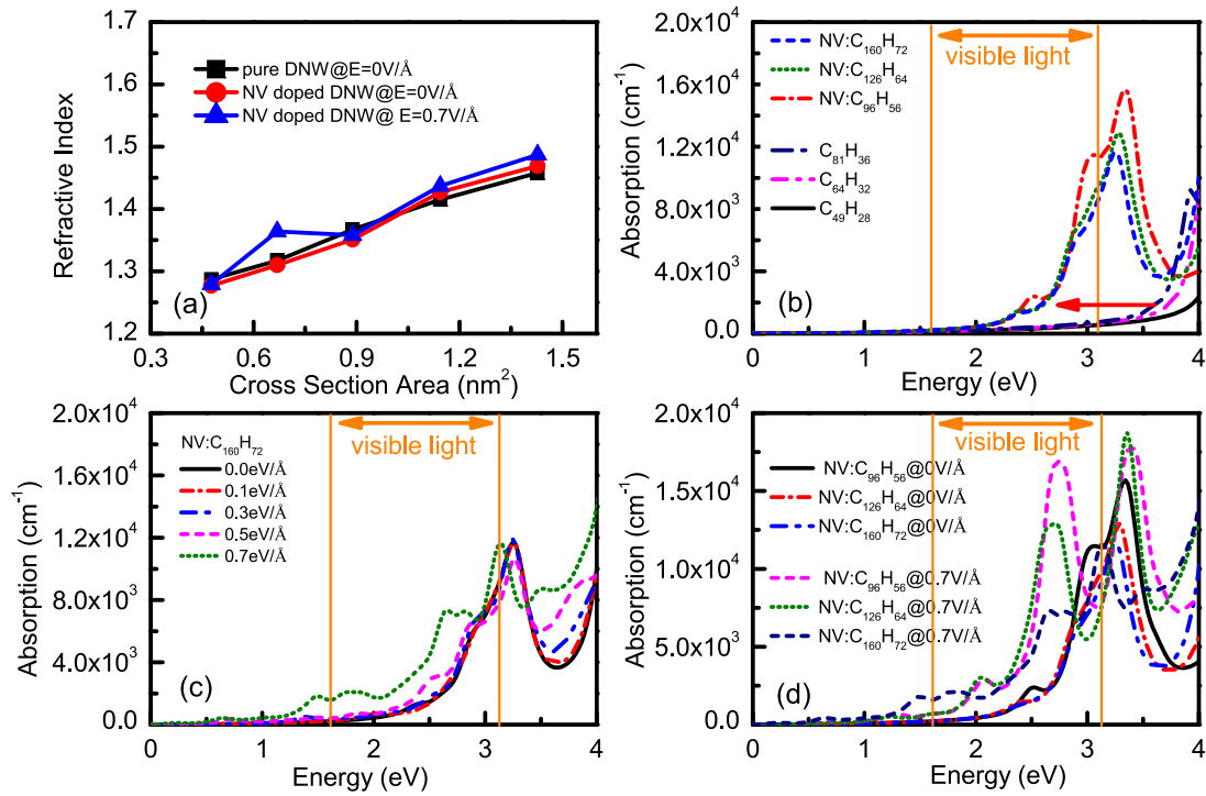
FIG. 4. (Color online) (a) The refractive index vs nanowire cross section area of the hydrogenated DNW under external electric fields \vec{E} of 0 and 0.7 \text{ V/Å} . (b) Absorption coefficients of \text{C}_{49}\text{H}_{28} , \text{C}_{64}\text{H}_{32} , \text{C}_{81}\text{H}_{36} , NV : \text{C}_{96}\text{H}_{56} , NV : \text{C}_{126}\text{H}_{64} , and NV : \text{C}_{160}\text{H}_{72} without external electric field. (c) Absorption coefficients of NV : \text{C}_{160}\text{H}_{72} under external electric fields \vec{E} of 0, 0.1, 0.3, 0.5, and 0.7 \text{ V/Å} . (d) Absorption coefficients of NV : \text{C}_{96}\text{H}_{56} , NV : \text{C}_{126}\text{H}_{64} , and NV : \text{C}_{160}\text{H}_{72} under \vec{E} = 0 and 0.7 \text{ V/Å} .
