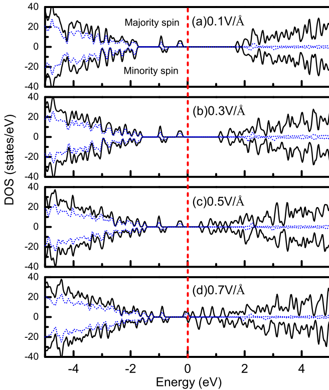
FIG. 2. (Color online) (a–d) DOS of NV : C 160 H 72 under external electric fields \vec{E} of 0.1, 0.3, 0.5, and 0.7 V/Å. The blue dotted lines show projections of the DOS onto C–2 p states. The upper and lower panels of each DOS plot represent the majority- and minority-spin channels, respectively. The Fermi level is indicated by the vertical dashed line.
