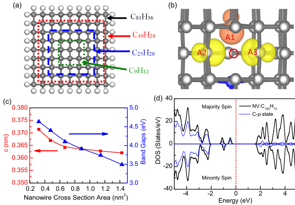
FIG. 1. (Color online) (a) The cross section of the hydrogenated diamond nanowires with C\{100\} surface. (b) Isosurface charge density plot (with an isovalue \rho = 0.02 e/\text{\AA}^3 ) of the spin states for NV : C_{160}H_{72} , showing the localized nature of defect states. C: gray; N: blue; C vacancy: red circle. (c) Lattice constants c (red square) and electronic band gap (blue triangle) vs the cross-sectional area of hydrogenated diamond nanowires. (d) DOS of NV : C_{160}H_{72} (black). The upper and lower panels of the DOS represent majority- and minority-spin channels, respectively. The blue dotted lines represent C-2p states of NV : C_{160}H_{72} . The Fermi level is indicated by the vertical dashed line.
