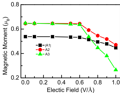
FIG. 3. (Color online) Local magnetic moments of A1, A2, and A3 atoms as a function of the external electric field \vec{E} .
