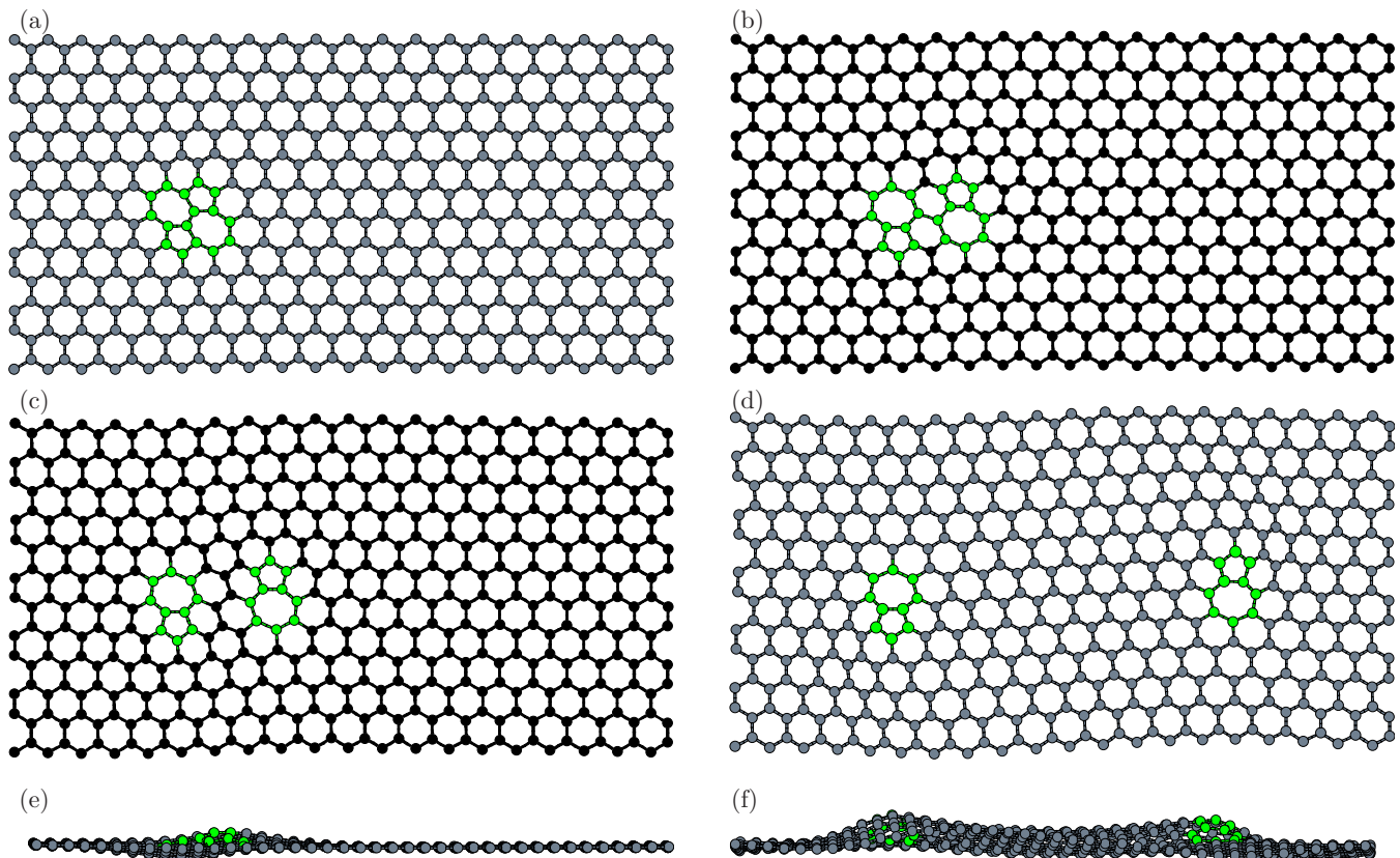
FIG. 6. (Color online) Step by step separation of the 5775 SW defect (a) into two 57 defects with one (b), two (c), and nine (d) hexagon pairs in between. Panels (e) and (f) are side views of the configuration in (a) and (d), showing much larger out-of-plane deformations for the case of separated 57 defects, due to strong stress in that case.
