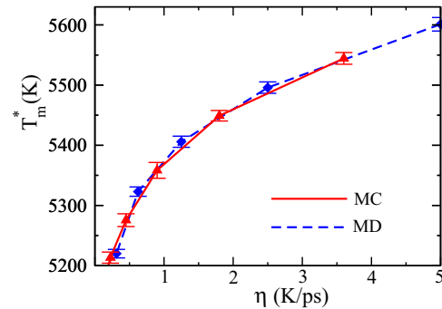
FIG. 2. (Color online) Comparison of the average, observed melting temperature, T_m^* , of bulk graphene (1008 atoms with PBCs) as a function of the heating rate obtained from MD (blue diamonds) and MC (red triangles) simulations after calibration, using LCBOP II without the middle range interactions. Error bars are based on 48 independent simulations. Lines are guides to the eye.
