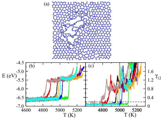
FIG. 1. (Color online) (a) Snapshot of simulated bulk graphene at the onset of melting. The system contains 1008 atoms with PBCs. Note the coexistence of solid and liquid parts. (b) Energy E and (c) order parameter \gamma_{12} as a function of temperature T during a linear temperature ramp for eight independent simulations.
