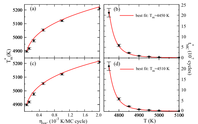
FIG. 3. (Color online) Symbols: (a) and (c) average melting temperature T_m^* as a function of the MC heating rate \eta_{\text{MC}} and (b) and (d) MC “time” t_{\text{MC}}^* required for melting at isothermal conditions as a function of temperature. The error bars are based on at least 48 independent simulations, but those for the isothermal simulations at 4750, 4800, and 4850 K are based on 96 simulations. The solid (red) curves represent simultaneous best fits of both sets of simulation data based on predictions by CNT [(a) and (b)] and KNT [(c) and (d)].
