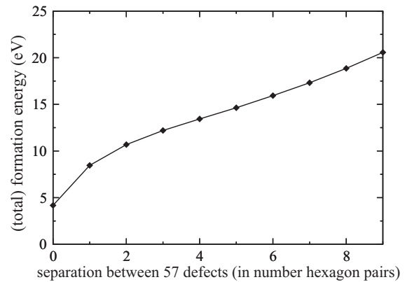
FIG. 7. Total formation energy as a function of the separation between 57 defects according to LCBOPII, calculated for the same sample as used for Fig. 6.
