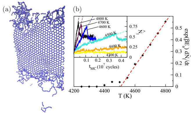
FIG. 5. (Color online) (a) Snapshot of a melting ribbon consisting of 2016 atom at T = 4500 K. (b) The simulated melting speed (symbols), \exp(\beta E_a) d\hat{N}_l/dt , as a function of the temperature T for a graphene ribbon. The inset shows the fraction of liquid particles \hat{N}_l as a function of t_{MC} for various simulation temperatures as indicated. For the completely liquid phase \hat{N}_l \simeq 0.5 as many particle still have a \gamma_{12} < 0.2 due to a rather isotropic neighbor surrounding.
