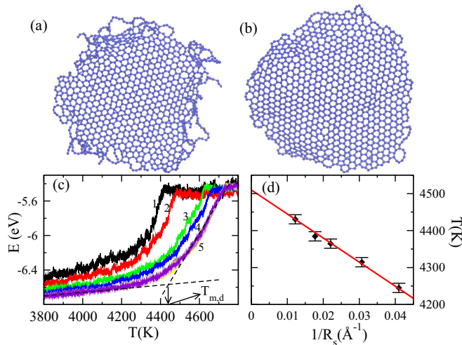
FIG. 4. (Color online) (a) Snapshot at 4300 K, illustrating edge melting of a graphene disk containing 1274 atoms heated at a rate of 2.5 \times 10^{-4} K/cycle. (b) Snapshot illustrating the recrystallization after cooling the system in (a) from 4300 to 3800 K. (c) Melting curves for different graphene disk sizes: (1) 714, (2) 1274, (3) 2470, (4) 3820, and (5) 8020 atoms. For the latter cluster, melting curves from four independent simulations are drawn but they are almost overlapping. The crossing dashed lines illustrate the method used to define the melting temperature T_{m,d} of a disk. (d) Best fit (red line) according to Eq. (7) of the average simulated disk melting temperatures (symbols). The error bars are based on four independent simulations.
