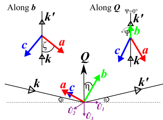
FIG. 9. (Color online) Schematic diagram of the x-ray diffraction experiment at zero azimuth ( \Psi = 0 ). k and k' are the incident and scattered x-ray beam wave vectors, and Q = k' - k is the scattering wave vector. The main (bottom) panel shows the orientation of the laboratory frame unit vectors \hat{U}_{1,2,3} and the orthorhombic crystal axes (a,b,c) . Top left inset: view along b showing the angle \zeta subtended from the scattering plane by the a vector. Right inset: view along Q . During an azimuth scan the crystal axes are rotated around Q by an angle \Psi (in the sense shown in the figure); the reference position \Psi = 0 is defined as the azimuth angle for which b lies in the scattering plane making the smallest angle with the incident beam direction \hat{k} .
