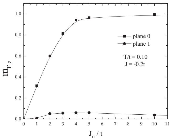
FIG. 11. Dependence of the ferromagnetic order parameter m_F for the itinerant spins as a function of the interaction J_H with a ferromagnetic Ising plane. We choose temperature T = t/10 . Here, t_{\perp} = t and J = -0.2t .
