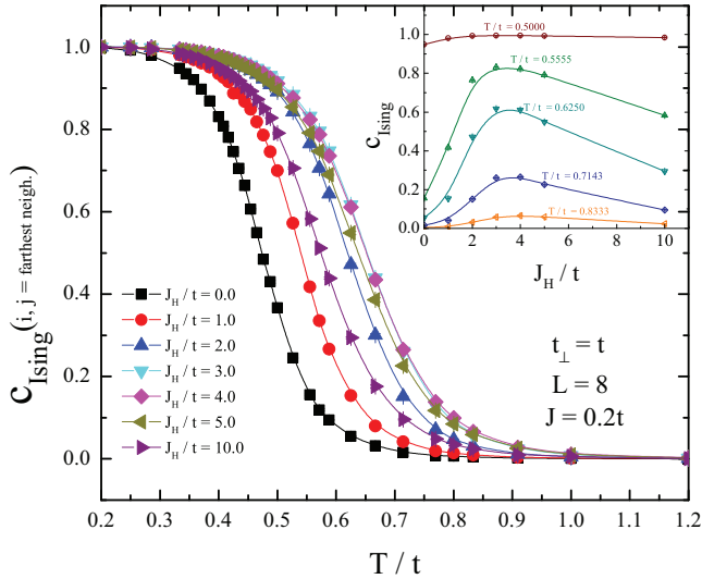
FIG. 4. (Color online) Temperature dependence of the Ising spin-spin correlation between most distant neighbors in the lattice and several values of the interaction J_H for L = 8 with one Ising layer stacked over two fermion ones. These correlations display a similar trend to the critical temperature: they initially become more robust with the coupling between the different planes; for large J_H , they return to values similar to the decoupled Ising model ( J_H = 0 ). The inset shows the same but now as a function of J_H where the nonmonotonic effects on the Ising spins correlations are unequivocal.
