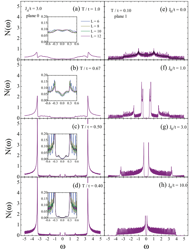
FIG. 9. (Color online) (Left) Density of states N(\omega) of fermions in plane 0 for different temperatures T/t = 1.00, 0.67, 0.50, 0.40 [(a)–(d)]. The linear lattice size L = 12 , Ising exchange coupling J = 0.2t , classical spin-fermion spin coupling J_H = 3t , and the interplane hopping t_{\perp} = t . There are two interesting features in N(\omega) : a pile-up of density at \omega \sim \pm J_H , which is present even at high T , and a gap which opens in the vicinity of \omega = 0 when T is decreased. Insets display the finite-size dependence around \omega = 0 . See text for further discussion. (Right) Density of states N(\omega) of fermions in plane 1 for different J_H/t = 0.0, 1.0, 3.0, 10.0 [(e)–(h)]. The temperature T/t = 0.10, t_{\perp} = t , and L = 12 . A gap is present for finite J_H , but gets filled for larger J_H . (See text for discussion.)
