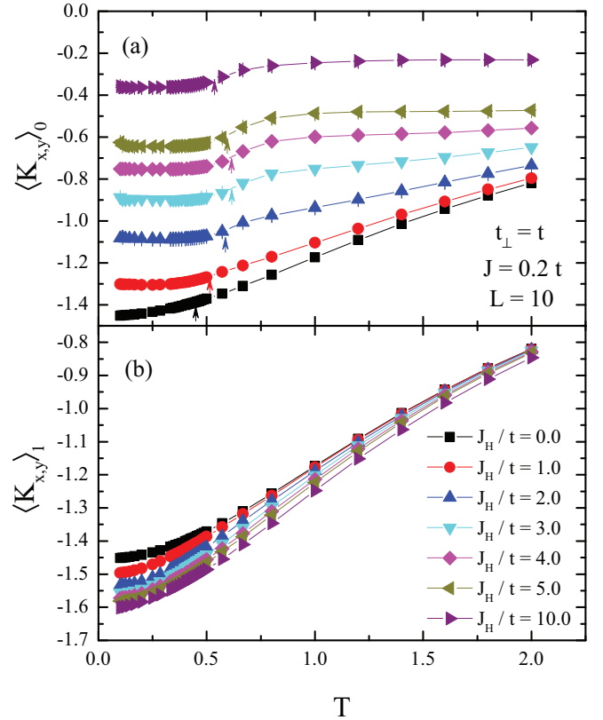
FIG. 5. (Color online) Intraplane kinetic energy \langle K \rangle as a function of temperature for different values of the interaction J_H . Here, t_\perp = t . In (a), the fermionic plane \ell = 0 directly in contact with the Ising spin layer; and in (b) the more distant fermionic plane \ell = 1 . The trend with increasing J_H is opposite in (a) and (b). For \ell = 0 , the connection to the Ising spins reduces the kinetic energy at all temperatures. For \ell = 1 , the kinetic energy increases. The vertical arrows at panel (a) indicate the critical temperature below which the magnetic ordering takes place for the Ising spins (Fig. 3).
