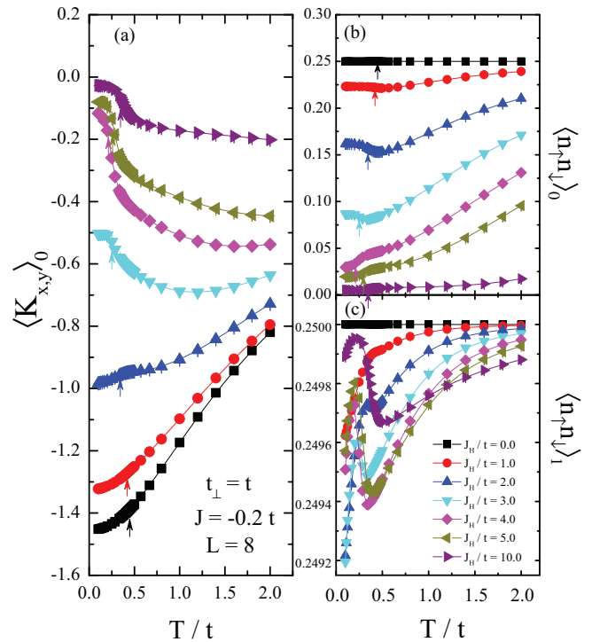
FIG. 12. (Color online) In (a), temperature dependence of the intraplane kinetic energy for \ell = 0 in the case t_{\perp} = t and ferromagnetic interaction between the Ising spins with exchange constant J = -0.2t . J_H/t \gtrsim 3.0 marks a distinct behavior where the kinetic energy decreases rapidly with decreasing temperature in opposition to the cases where J_H is small. Equivalently to Fig. 6, the temperature dependence of the double occupancy in planes \ell = 0 and \ell = 1 , (b) and (c), respectively. In the former, similar to the antiferromagnetic case, the increase in moment localization due to the interaction with the neighbor Ising spins can be readily seen. In the latter, despite the upturn of double occupancy for low temperatures and large interactions, the later downturn for even smaller temperatures indicates that the ferromagnetism of the Ising layers starts to propagate through the more distant fermionic region. Again, in (a) and (b), the vertical arrows depict the Ising critical temperature T_c .
