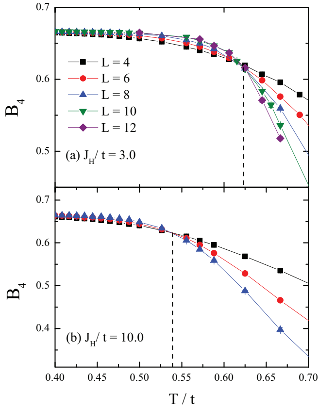
FIG. 2. (Color online) Crossing plot of the Binder ratio of an AF Ising sheet coupled with J_H = 3t (top) and J_H = 10t (bottom) to two metallic layers. The interlayer hopping between the fermion layers was set to t_\perp = t . For J_H = 3t , the crossing occurs at T/t \sim 0.62 , which is well above the critical temperature of a free Ising sheet ( J_H = 0 ). T/t = (J/t) \times (T_c/J) = 0.2 \times 2.269 = 0.454 . The behavior of T_c with J_H is nonmonotonic as the critical temperature for J_H = 10t drops to T/t \sim 0.54 (see Fig. 3).
