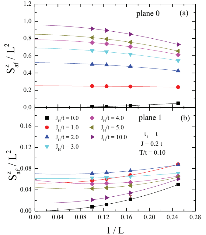
FIG. 7. (Color online) Finite-size extrapolation for the z component of the antiferromagnetic structure factor S_{af}^z for planes 0 and 1, in (a) and (b), respectively. Here, t_{\perp} = t and T/t = 0.10 . A parabolic fit is used to obtain the value in the thermodynamic limit, m_{af,z}^2 .
