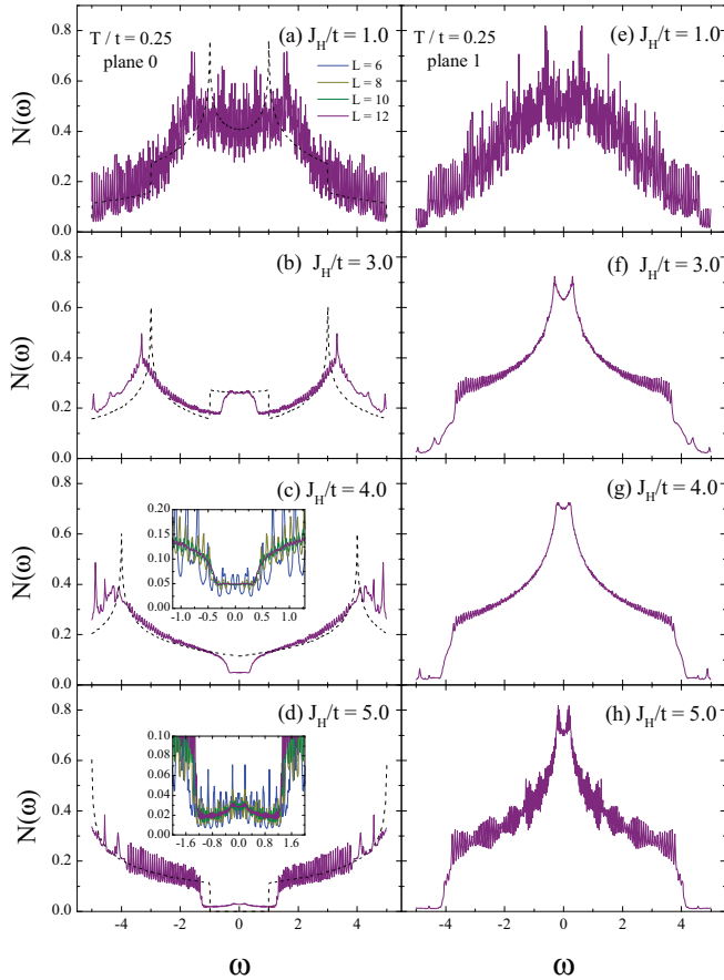
FIG. 13. (Color online) Density of states N(\omega) of fermions in plane \ell = 0 for different values of the interaction J_H/t = 1.0, 3.0, 4.0, 5.0 [(a)–(d)] at temperature T/t = 0.25 . [(e)–(h)] show the correspondent results for plane \ell = 1 . The linear lattice size is L = 12 , Ising exchange coupling J = -0.2t and the interplane hopping t_{\perp} = t . Insets at (c) and (d) include also L = 6, 8 , and 10 near the region \omega = 0 . Also displayed, as a dashed line, the corresponding density of states resulting from the dispersion of one plane under the influence of a fixed global chemical potential as if the configuration for the Ising spins is “frozen” in the ferromagnetic state. Worth noting is that there is a pile-up of density at \omega \sim \pm J_H , and a pseudogap, which opens only for values of J_H/t \gtrsim 4 . Insets in (c) and (d) show a finite-size comparison of this gap.
