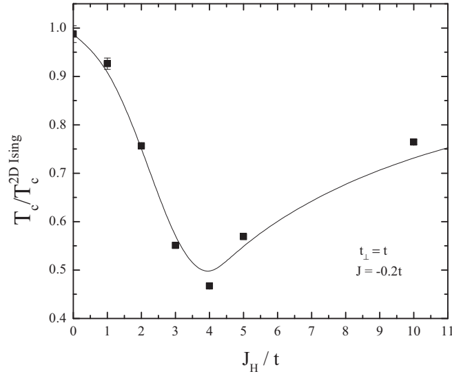
FIG. 10. Curie temperature for the ferromagnetic Ising model with J = -0.2t coupled with two fermionic planes ( t_{\perp} = t ), as a function of J_H . Unlike the antiferromagnetic case, the coupling with metal decreases the ferromagnetic critical temperature. Lines are guides to the eye.
