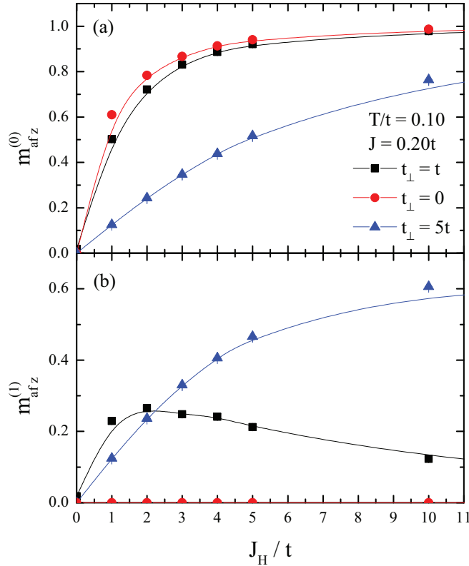
FIG. 8. (Color online) Antiferromagnetic order parameter as a function of J_H for temperature T/t = 0.10 . In (a) for plane 0 and in (b) the same for plane 1. Plane 0 exhibits a rapid and monotonic saturation with J_H . m_{af,z}^{(1)} in plane 1 first increases with J_H and then falls.
