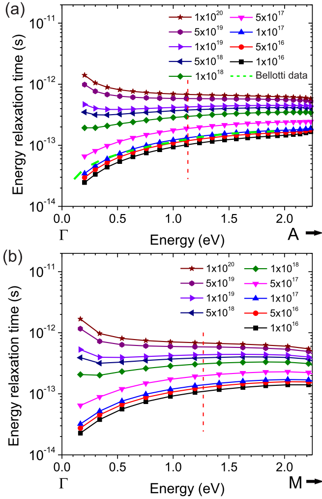
FIG. 4. (Color online) Calculated energy relaxation time due to an electron-LO-phonon interaction for electrons in the CB of GaN along (a) \Gamma -A and (b) \Gamma -M directions. The curves are given for various carrier concentrations (in \text{cm}^{-3} ). The vertical dashed lines denote the energies of inflection points. The Bellotti data are from Ref. [17].
