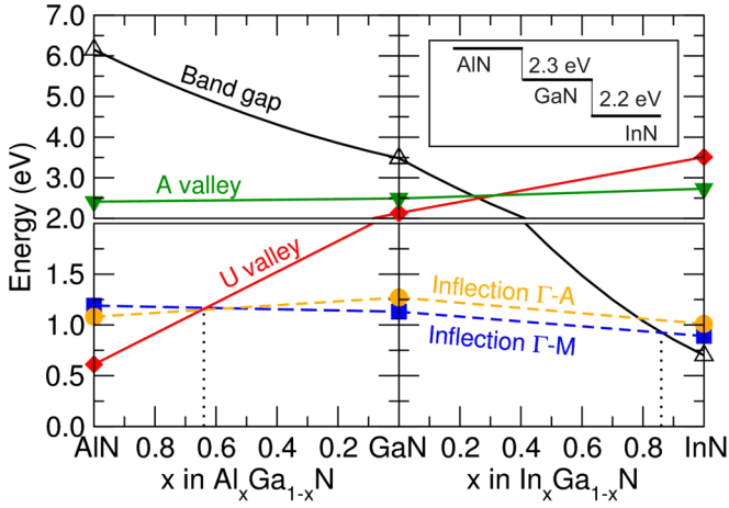
FIG. 3. (Color online) Band-structure-related quantities for AlN, GaN, and InN, as well as AlGaIn and InGaIn alloys: experimental band gaps, and energies of inflection points and of U and A valleys, referenced to the CBM. Note the change in scale between lower and upper panels. The vertical dashed lines denote crossing points between physical quantities relevant for NDR. The inset shows the CB offsets between the CBM (at \Gamma ) in AlN, GaN, and InN (from Ref. [29]).
