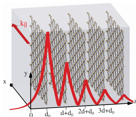
FIG. 1. (Color online) Geometry of the problem: a truncated multilayer structure composed of graphene sheets separated by the dielectric layers with permittivity \varepsilon and thickness d . A thin dielectric layer of the thickness d_0 is a cap layer. The external dielectric has permittivity \varepsilon' . The red curve shows an example of a profile of the surface mode (shown is the tangential electric field component).
