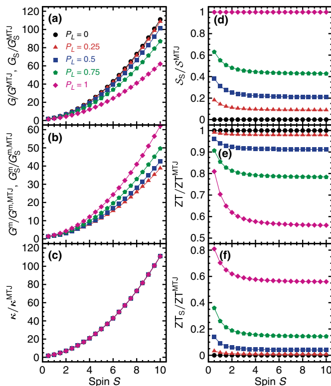
FIG. 3. (Color online) Diagonal (a) and nondiagonal (b) elements of the conductance matrix \mathbf{G} , electronic contribution to the heat conductance \kappa (c), spin thermopower \mathcal{S}_S (d), figure of merit ZT (e), and spin figure of merit ZT_S (f) shown as functions of the impurity spin number S for several values of the left electrode's spin-polarization parameter P_L . Note that the points correspond to spin numbers while the lines serve merely as a guide for eyes. Remaining parameters: T = 1 K, x_R = 10 eV ^{-1} , \alpha_d = \alpha_{\text{ex}} = 1 , \lambda = 1 , and \nu_L = \nu_R = 1 , so that \mathcal{A} = 1 (i.e., the junction is fully symmetric with respect to DOS and exchange coupling).
