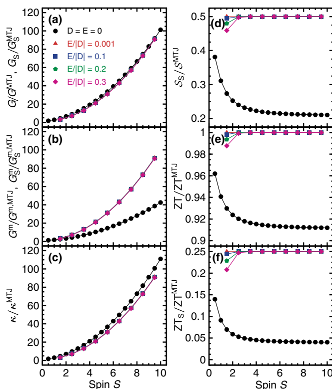
FIG. 6. (Color online) Analogous to Fig. 3, but now the quantities under consideration are plotted for the case of an anisotropic spin impurity with D = 100 \mu\text{eV} and indicated values of the transverse magnetic anisotropy E . Except P_L = 0.5 and T = 0.1 \text{ K} , all parameters are as in Fig. 3. For comparison, black dots representing the situation of an isotropic ( D = E = 0 ) spin impurity are also presented.
