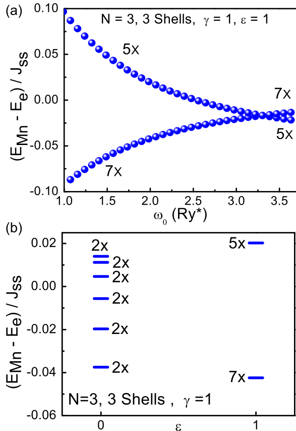
FIG. 4. (Color online) (a) Evolution of the energies of three-electron levels with J = 3 and J = 2 as a function of the QD shell spacing \omega_0 . (b) Energy difference \Delta for both anisotropic ( \epsilon = 0 ) and isotropic ( \epsilon = 1 ) e -Mn interactions in a three-shell QD with full interactions ( \gamma = 1 ).
