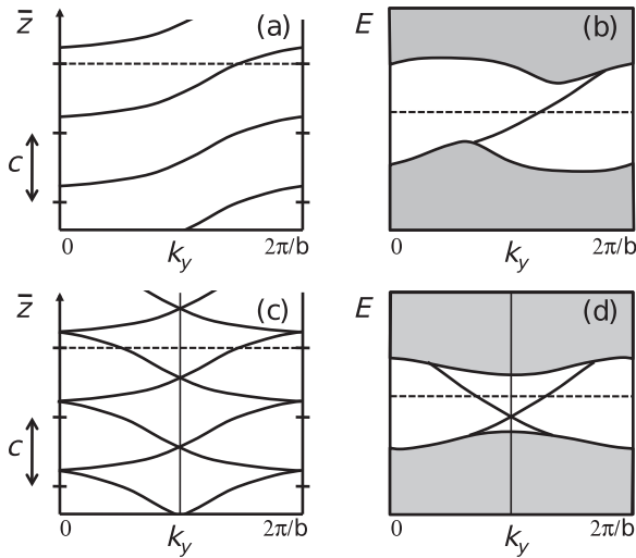
FIG. 1. (a) Flow of Wannier charge centers along \hat{z} vs k_y for a 2D Chern insulator. (b) Flow of surface energy bands vs k_y for a 2D Chern insulator. (c), (d) Same, but for a 2D Z_2 -odd (quantum spin Hall) insulator. Dashed lines are arbitrary reference positions in (a) and (c), or Fermi energies in (b) and (d).
