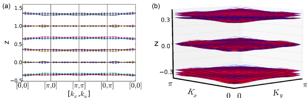
FIG. 4. (Color online) First-principles WCC sheets along \hat{z} for topologically trivial \text{Sb}_2\text{Se}_3 , plotted on (a) the boundary and (b) the interior of the 2D quarter BZ. The WCCs show trivial behavior as expected.
