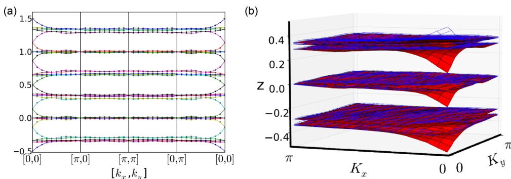
FIG. 8. (Color online) First-principles WCC sheets for the strong TI \text{Bi}_2\text{Se}_3 , plotted on (a) the boundary and (b) the interior of the 2D quarter BZ. The WCC sheets on parallel TRI faces (e.g., at k_x = 0 and \pi ) show opposite topological behavior.
