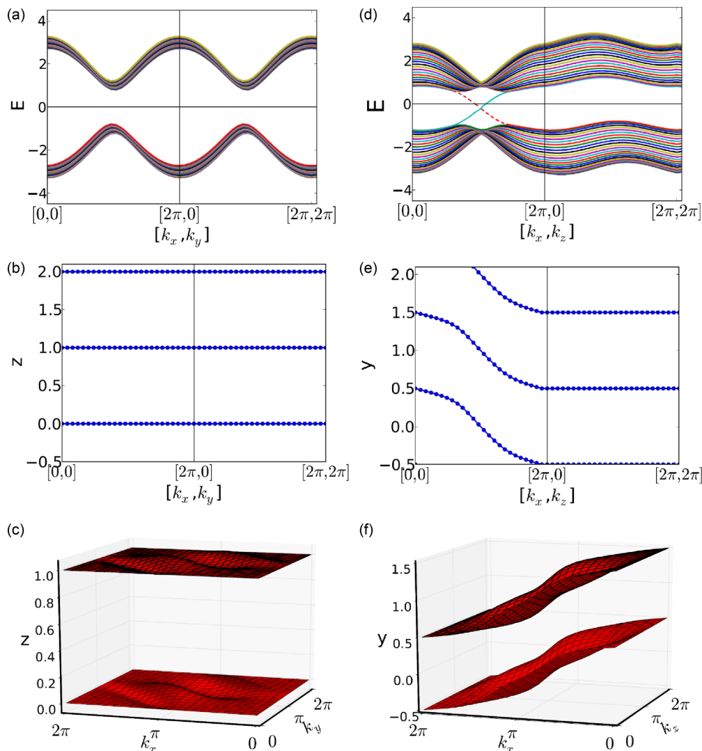
FIG. 2. (Color online) Surface energy bands and WCC sheets for the TR-broken Chern insulator model. (a)–(c) Surface normal and WCCs along \hat{z} vs (k_x, k_y) . (d)–(f) Surface normal and WCCs along \hat{y} vs (k_x, k_z) . Surface states for a 24-layer slab in (a) and (d); WCCs around 2D BZ boundary in (b) and (e); WCCs in 2D BZ in (c) and (f). Dashed and solid surface states in (d) reside on the top and bottom of the (010) slab, respectively. The WCC sheets and surface bands wind by one unit in the k_y - k_z plane, but not in the k_x - k_y plane.
