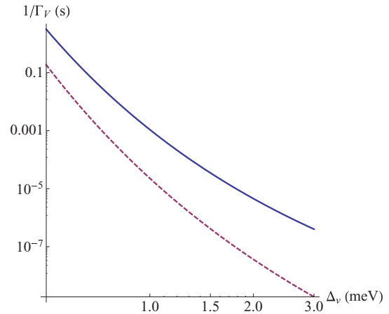
FIG. 10. (Color online) Total valley relaxation time (due to both transverse and longitudinal phonons) for an ideal interface, quantum dot excited valley state in silicon versus valley splitting, \Delta_v . The exact results including all multipole contributions are given by the blue solid line while ED approximation (see text) results are given by the purple dashed line. Typical valley splittings in silicon quantum dots are less than 1 meV.
