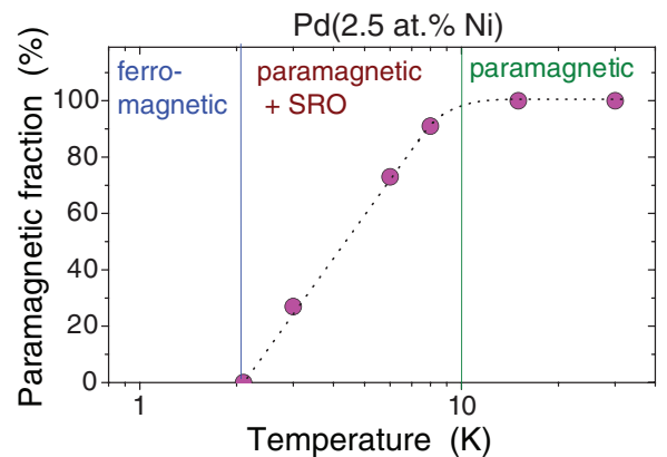
FIG. 15. (Color online) Schematic phase diagram of the magnetic states of Pd (2.5 at.% Ni).
