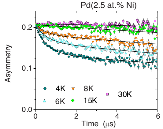
FIG. 14. (Color online) ZF- \mu\text{SR} asymmetry data from the 2.5 at.% Ni alloy above 2 K. The spectra at 4, 6, and 8 K were fitted with the sum of rapidly- and slowly-relaxing exponential components; the data at 15 and 30 K with a slowly relaxing exponential only. The data were obtained using the GPS spectrometer.
