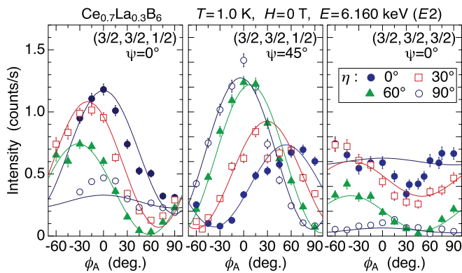
FIG. 4. (Color online) \phi_A dependencies of the E_2 intensity at zero field in phase IV. The incident polarization angle \eta is fixed and \phi_A is scanned. Solid lines show the calculated intensity curves assuming the \Gamma_{5u} -type AFO order of (\pm T_x^\beta \pm T_y^\beta \pm T_z^\beta) with four equal domain populations.
