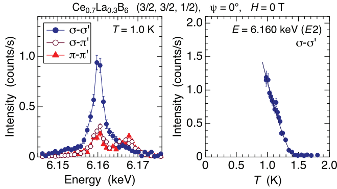
FIG. 3. (Color online) (Left) X-ray energy dependence of the intensity for \sigma - \sigma' , \sigma - \pi' , and \pi - \pi' channels. (Right) Temperature dependence of the E_2 resonance intensity at 6.160 keV for the \sigma - \sigma' channel. The solid line is a fit to a power law I \propto |T - T_{IV}|^{2\beta} with \beta = 0.70 \pm 0.1 .
