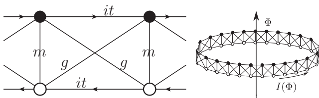
FIG. 2. Left: Creutz model in zero flux on a linear infinite lattice. The horizontal ladders represent symbolically the two spin projections: the upper (lower) ladder with filled (empty) circles denotes \sigma_3 spin-up (spin-down) states. The spin degeneracy is lifted by an on-site coupling m . There are two possible hopping amplitudes: the g term that produces spin-flip processes and a spin-conserving hopping t . The additional phase \pi/2 on the t links is only conventional and has the role to move the Dirac point at k = 0 . Right: The model is shaped into a ring of length L and a flux \Phi is threaded through it.
