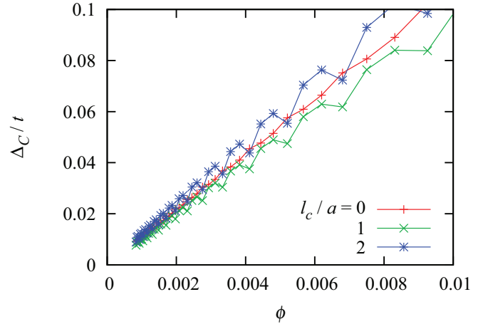
FIG. 3. (Color online) Influence of finite-range interactions on \Delta_C is shown for U/t = 10 , V/t = 1 , and various values of the cutoff distance, l_c , in the off-site interaction. The other parameters are the same as in Fig. 2.
