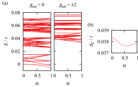
FIG. 4. (Color online) \alpha dependence of the energy spectrum for the sectors of \chi_{\text{tot}} = 0 and \chi_{\text{tot}} = \pm 2 (a) and the charge gap (b). The parameters are the same as in Fig. 1.
