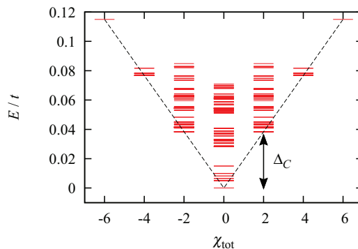
FIG. 1. (Color online) Energy spectrum classified according to the total chirality \chi_{\text{tot}} in the Ising limit \alpha = 0 , for M = 3, \phi = 1/300, U/t = 10 , and J/t = 1 . The spectrum is symmetric about \chi_{\text{tot}} = 0 , and the bottoms of different sectors exhibit a linear increase with |\chi_{\text{tot}}| as indicated by dashed lines.
