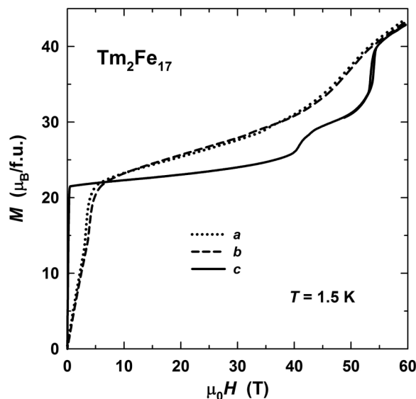
FIG. 8. Magnetization curves in pulsed magnetic fields applied along the principal axes of a \text{Tm}_2\text{Fe}_{17} single crystal.
