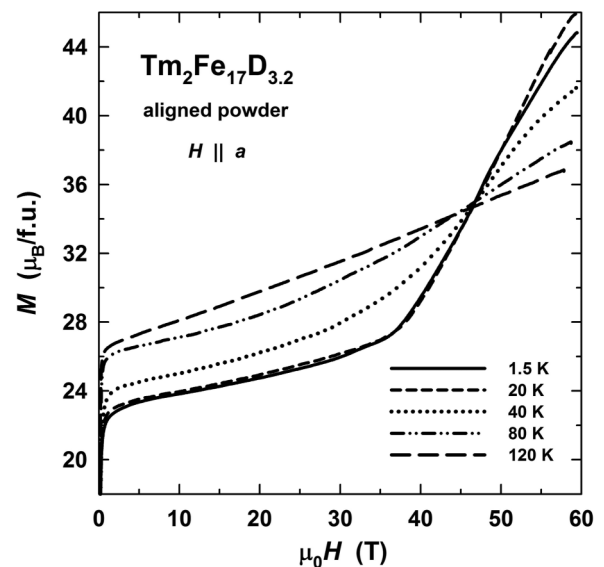
FIG. 12. Temperature evolution of the magnetization curve of \text{Tm}_2\text{Fe}_{17}\text{D}_{3.2} (sample a ).
