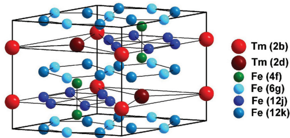
FIG. 1. (Color online) Crystal structure of \text{Tm}_2\text{Fe}_{17} .
