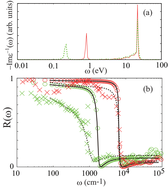
FIG. 2. (Color online) (a) Calculated energy loss function of (TMTSF) 2 PF 6 . The red-solid and green-dotted curves represent the spectra for E \parallel a and E \parallel b' , respectively. (b) Ab initio reflectivity (circles) and experimental one (crosses) at 25 K (Ref. 7). The results for E \parallel a and E \parallel b' are displayed by dark red and light green, respectively. The solid and dotted curves are the fits by Eq. (11) with parameters shown in Table I.
