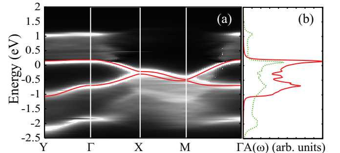
FIG. 3. (Color online) (a) Calculated spectral function A(\mathbf{k},\omega) of (TMTSF) 2 PF 6 , superposed by the Kohn-Sham band structure (red curves). The Fermi level is at zero energy. (b) Density of states obtained by KS (red-solid curve) and GW (green-dotted curve).
