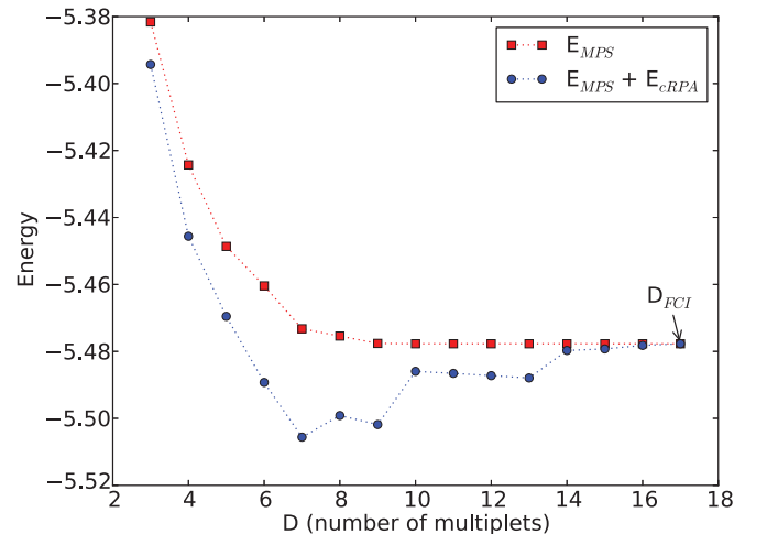
FIG. 1. (Color online) The RPA-MPS correlation energy for the Hubbard chain with OBC, length L = 6 , filled with N = 4 electrons, in the singlet state, and U = 1 . A symmetry-adapted Ansatz was used, with D retained multiplets at each boundary.
