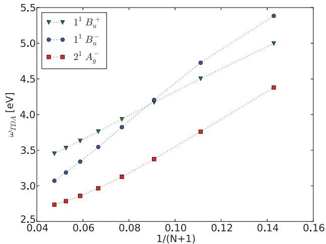
FIG. 2. (Color online) The first three TDA-MPS excitation energies for a polyene chain with N carbon atoms for which the \pi system was approximated by the long-range PPP Hamiltonian.
