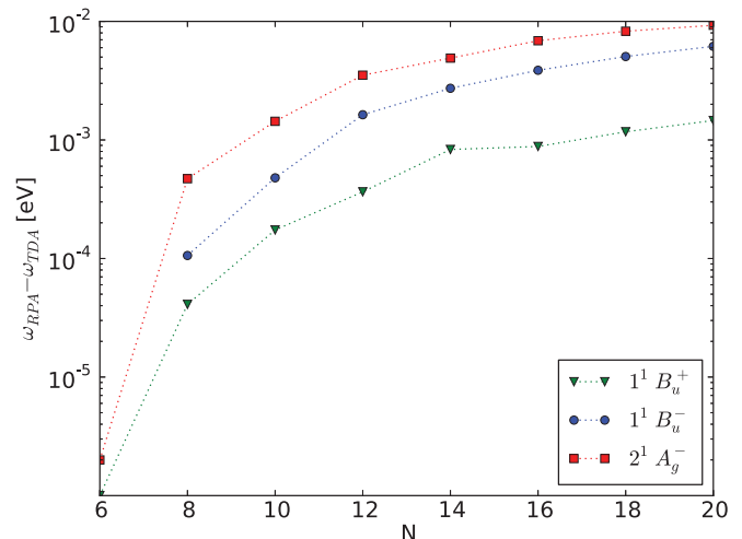
FIG. 3. (Color online) The difference between the RPA-MPS and TDA-MPS energies for the first three excitations of a polyene chain with N carbon atoms for which the \pi system was approximated by the long-range PPP Hamiltonian.
