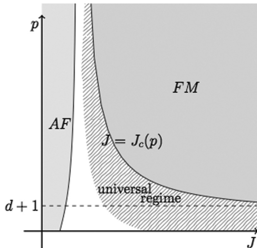
FIG. 1. Ground state phase diagram as a function of the antiferromagnetic decay exponent p and of the ferromagnetic strength J . In the leftmost region the ground state is the Néel antiferromagnetic state, while in the rightmost region it is the homogeneous ferromagnetic state. These two phases are rigorously known, while the rest of the phase diagram remains to be understood. The light-gray shaded region is the “universal regime,” where the ferromagnetic islands (droplets) have a typical size much larger than the lattice spacing. The conjecture is that the ground state is periodic and striped in the whole universal regime. A partial proof of this fact is given in this paper.
