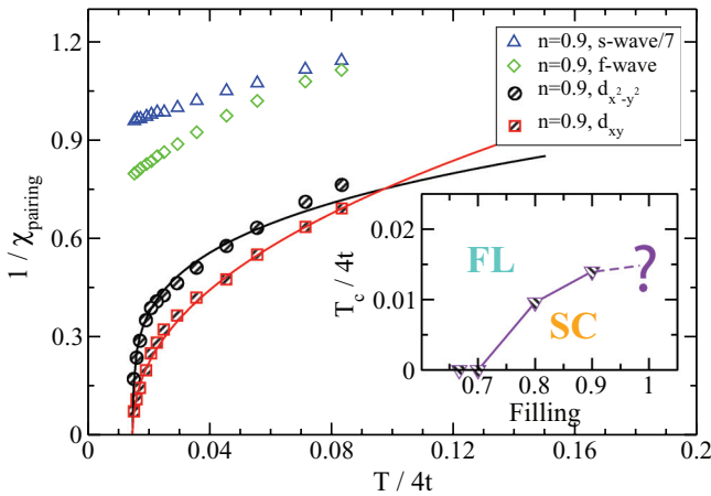
FIG. 3. (Color online) Inverse pairing susceptibility 1/\chi_{\text{pairing}} for N_c = 6 , U = 8.5t , and n = 0.9 . The singlet s wave and triplet f wave do not diverge, whereas the singlet pairing channels with d_{x^2-y^2} - and d_{xy} -wave symmetry show a divergency at the same T_c . Note that we have multiplied by a factor of 7 the s -wave pairing susceptibility in order to use the same vertical scale. Inset: The superconducting transition temperature T_c as a function of doping. FL and SC label the Fermi liquid and superconducting regions, respectively. The nature of the system is still unclear at half filling, hence a question mark in the inset.
