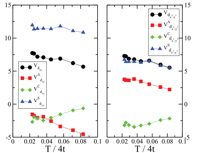
FIG. 4. (Color online) Left: d_{xy} projected contributions to the pairing vertex V_{d_{xy}} , from the fully irreducible vertex V_{d_{xy}}^A , charge V_{d_{xy}}^C , and spin V_{d_{xy}}^S cross channels vs T at n = 0.9 , U = 8.5t . Right: The d_{x^2-y^2} -wave projection of the same quantities. In both cases, the contribution to the pairing interaction from spin channel is clearly dominant.
