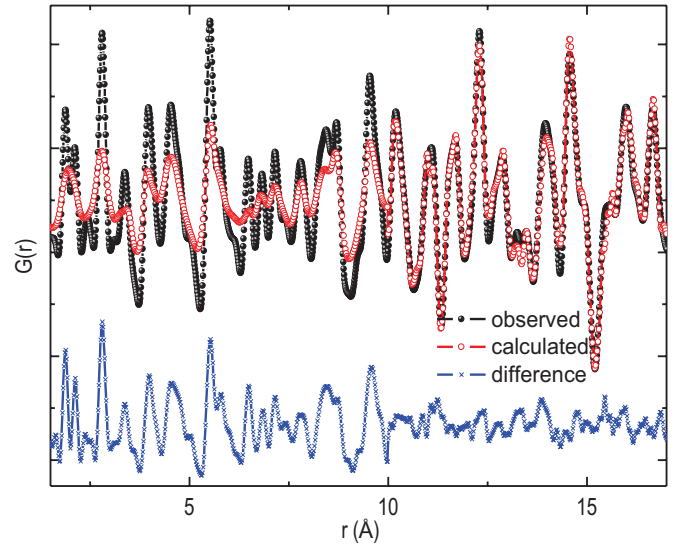
FIG. 9. (Color online) Neutron PDF analysis of NaNbO 3 at 15K with R3c and Pbcm group coexistence model from the Rietveld analysis. Note that the differences gradually vanish above 10 Å.
