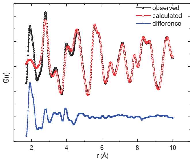
FIG. 4. (Color online) Neutron pair distribution function G(r) analysis of \text{NaNbO}_3 at 490 K with the Pbcm group. Note that this structure model can describe the PDF only above 5.2 Å.
