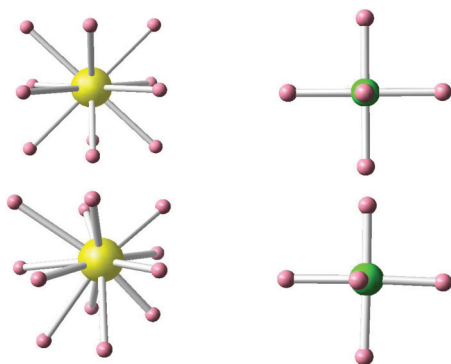
FIG. 8. (Color online) Depictions of NaO 12 at 930 K (left top) and at 15 K (left bottom), and NbO 6 at 930 K (right top) and at 15 K (right bottom) according to the PDF analysis. Na and Nb displacements are exaggerated for clarity.
