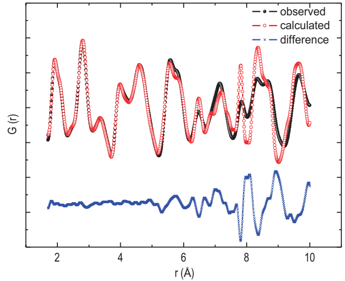
FIG. 5. (Color online) Neutron pair distribution function G(r) analysis of \text{NaNbO}_3 at 490 K with the R3c group. Note that this phase can describe the structure profile only below 5.2 Å.
