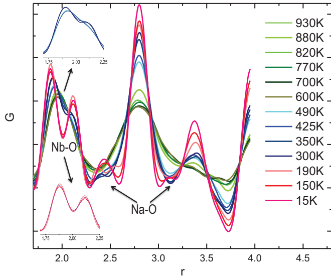
FIG. 7. (Color) Neutron pair distribution function G(r) analysis of NaNbO 3 from 930 to 15 K up to 4 Å. Note that the result can be divided into three groups with the evolution of temperature: 900–600 K (green lines), 490–300 K (blue lines), and 190–15 K (red lines). This indicates that only two basic structural changes happen at a short range. Peaks resulted from Na-O and Nb-O bonds are marked with arrows and obvious Nb-O bond lengths changes at very short distance from 490 to 15 K are also emphasized in the inset.
