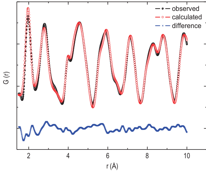
FIG. 3. (Color online) Neutron pair distribution function G(r) analysis of \text{NaNbO}_3 at 820 K with the Cmc parameters from the Rietveld analysis. This phase is well described by the Cmc structure. Models obtained by the Rietveld analysis can fit the PDF from 930 to 600 K quite well. This is an example that shows the accuracy of the Rietveld model at high temperatures.
