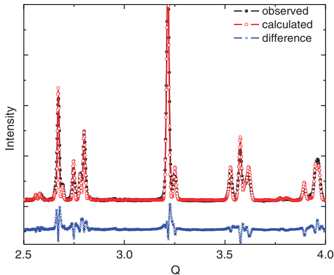
FIG. 2. (Color online) Observed (solid spheres), calculated (open circles), and difference (crosses) profiles obtained after the Rietveld refinement of \text{NaNbO}_3 using the mixture of phases with rhombohedra R3c group (70%) and orthorhombic Pbcm group (30%) at 15 K. Peaks marked with arrows are the ones belong only to the R3c group according to the analysis of GASA software.
