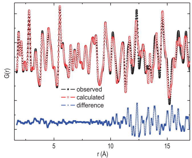
FIG. 10. (Color online) Neutron pair distribution function G(r) analysis of NaNbO 3 at 15 K with only the R3c group. Note that the differences are very small below 10 Å and begin to become obvious above 10 Å.
