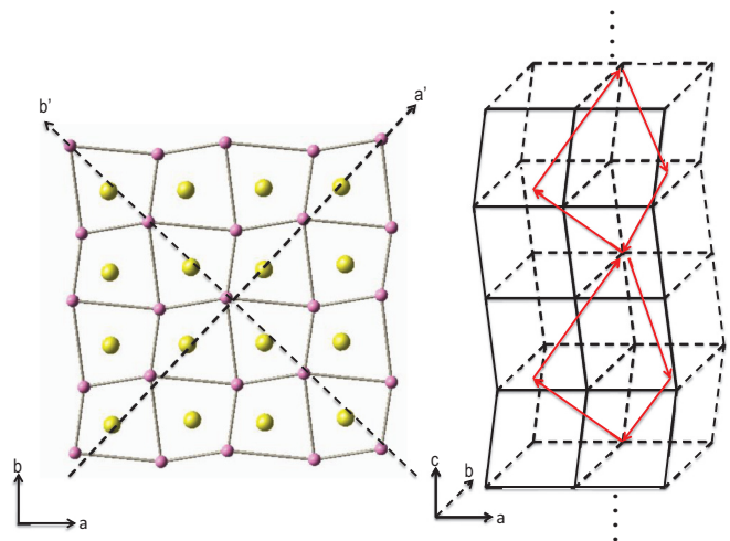
FIG. 6. (Color online) (a) Atomic arrangement of \text{NaNbO}_3 at 490 K. Yellow balls are Na, green balls are niobium, and purple balls are oxygen. a and b are R3c axes and a' and b' are Pbcm axes. (b) Construction of the basic cells ( \sim 4 Å) and local polarizations. Every arrow corresponds to a spontaneous polarization in an elementary perovskite cell.
