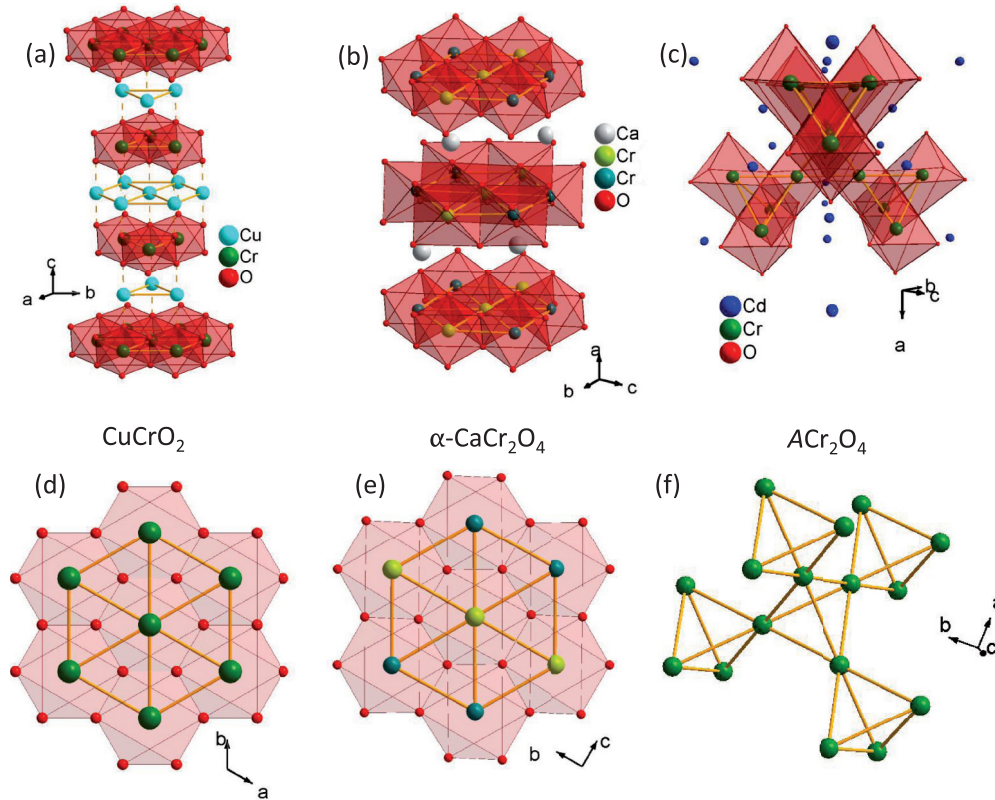
FIG. 1. (Color online) Room-temperature crystal structures of (a) \text{CuCrO}_2 , (b) \alpha\text{-CaCr}_2\text{O}_4 , and (c) \text{ACr}_2\text{O}_4 with A = \text{Cd, Zn} . In (d)–(f) we show the respective triangular planes and the pyrochlore lattice formed by the Cr ions in these compounds.
