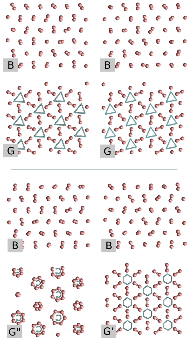
FIG. 4. (Color online) Time-averaged (1 ps) atomic positions from simulations at pressure/temperature/initial configuration. Top: Phase IVa, stacked BGBG , 220 GPa, 220 K, Pc . Bottom: Phase IVb, stacked BG'BG'' , 270 GPa, 220 K, Pc . The time averaging was chosen large enough to capture the rotation of the B -layer molecules and G'' -layer motifs, making these smaller. After a long time and complete rotations, the motifs become degenerate points at the central position representing 2 B and 6 G'' atoms, respectively. The G' -layer image is time invariant. Note the strong sixfold symmetry in phase IVb compared with IVa. Many other similar figures are given in the Supplemental Material, 33 showing the trends with P and T .
