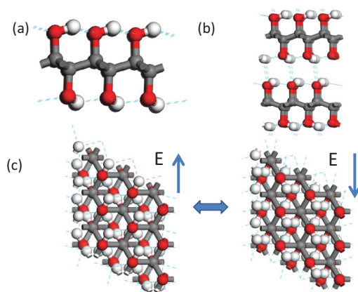
FIG. 2. (Color online) (a) Side view of single-layer HLGAs, (b) multilayer HLGAs, and (c) top view of multilayer HLGAs.
