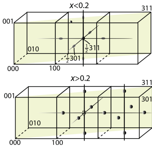
FIG. 2. (Color online) Representative \langle 310 \rangle selected area electron diffraction patterns for a series of (1-x)\text{NBT}-x\text{KBT} compositions. The superlattice reflections change from 1/2\{ooo\} for x < 0.2 to 1/2\{ooe\} for x > 0.2 . For x = 0.2 , both types of reflections are present though the dominant type varies from grain to grain. For x < 0.2 , the diffuse spots at 1/2\{ooe\} , which are streaked along \langle 100 \rangle directions, signify short-range ordered in-phase tilting. In contrast, for x \geq 0.2 , the round-shaped diffuse spots at 1/2\{ooo\} arise from intersections of several \langle 100 \rangle diffuse rods associated with 1/2\{ooe\} reflections, as discussed in the text. The reciprocal lattices for both cases are illustrated in the figure.
