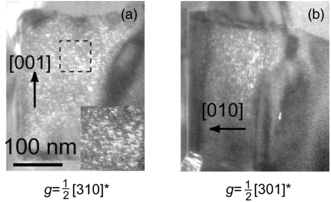
FIG. 8. A pair of dark-field images of the same area in a single grain x = 0.3 recorded using 1/2310 and 1/2301 reflections. The domains are textured along (a) [001] and (b) [010] directions. These images confirm that the same area contains at least two of the domain variants associated with 1/2\{00e\} reflections.
