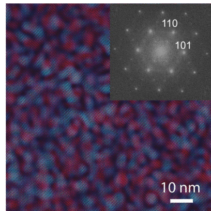
FIG. 9. (Color online) A colored overlay of the two \langle 111 \rangle HRTEM images of the same T1 domain ( x = 0.3 ), each obtained by Fourier filtering a raw image using a distinct set of 1/2110 -type reflections visible in the FFT pattern (inset). A given set of these superlattice reflections corresponds to one of the two domains (red or blue), which appear as spatially separate regions.
