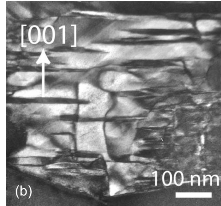
FIG. 3. (a) A dark field image of a single grain x = 0.1 reveals antiphase domain boundaries associated with octahedral tilting. (b) A dark-field image of another single grain in the same sample, which features both twin and antiphase domain boundaries. The twin boundaries reside largely on \{100\} planes. Both images were recorded with 1/2\{ooo\} reflections strongly excited near the \langle 310 \rangle orientation.
