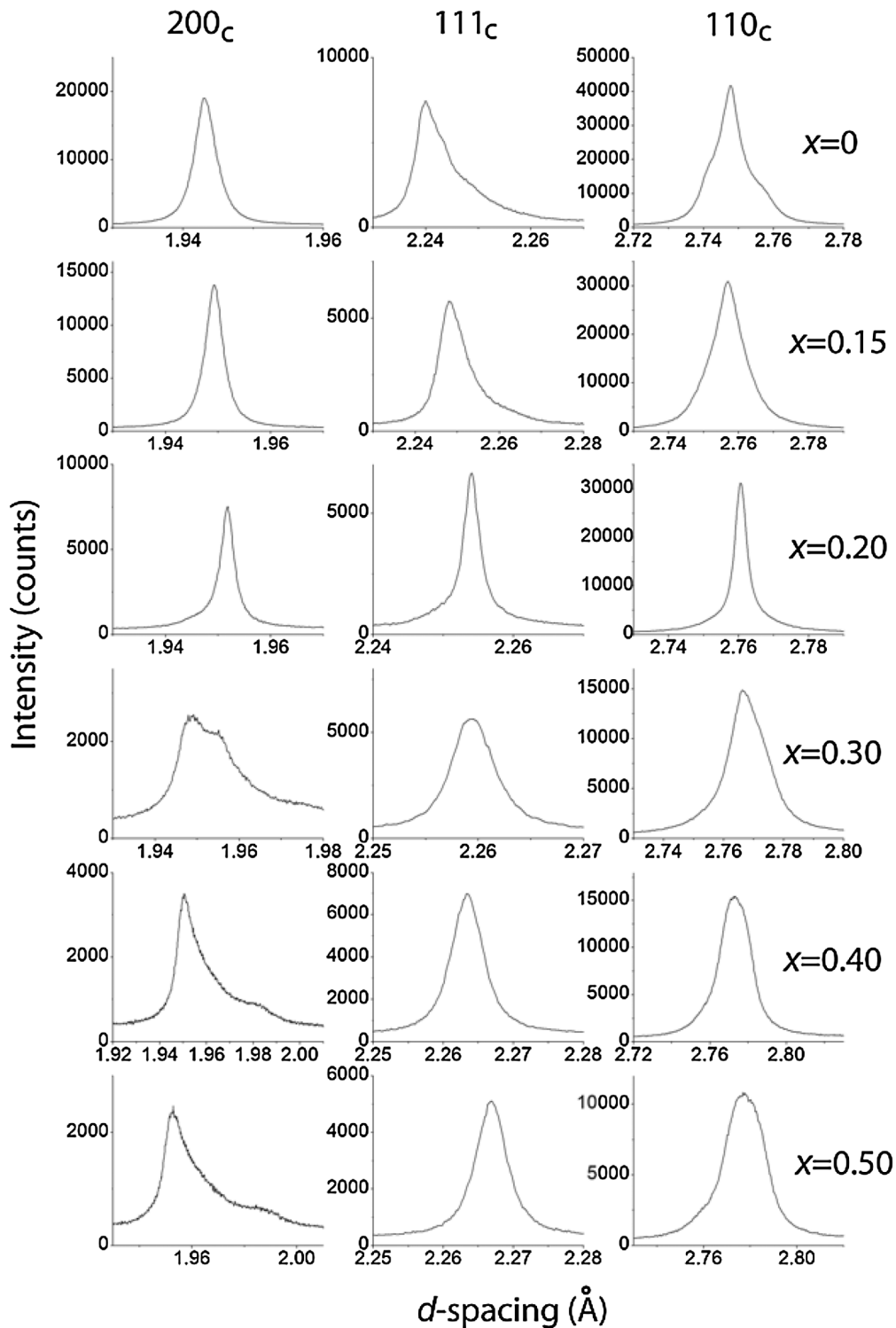
FIG. 1. Traces of 200, 111, and 110 x-ray diffraction reflections (synchrotron data) for several (1-x)\text{NBT}-x\text{KBT} compositions. Peak splitting is consistent with pseudorhombohedral and pseudotetragonal symmetries for x < 0.2 and x > 0.2 , respectively. The profiles for x = 0.1 are similar to those for x = 0 and therefore were omitted from this figure. The lattice distortion is minimal at the MPB ( x = 0.2 ), which creates the appearance of a cubic structure.
