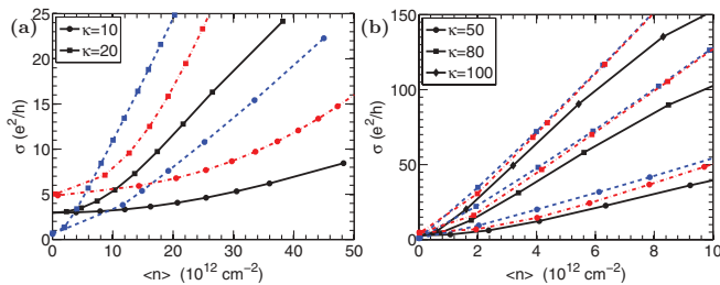
FIG. 10. (Color online) Calculated conductivity as a function of carrier density for different values of the substrate dielectric constant with the impurity density n_{\text{imp}} = 4.0 \times 10^{13} \text{ cm}^{-2} , d = 0.1 nm. The solid, dashed, and dot-dashed lines are obtained by using the TFD-EMT method, self-consistent method, and quasi-TFD method, respectively.
