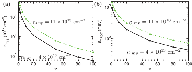
FIG. 5. (Color online) TFDT results at the CNP for d = 0.1 nm. (a) n_{rms} as a function of substrate dielectric constant \kappa . (b) Root mean square of the screened disorder potential s_{TFDT} as a function of substrate dielectric constant \kappa . The solid lines are for n_{imp} = 4 \times 10^{13} \text{ cm}^{-2} and the dashed lines are for n_{imp} = 11.0 \times 10^{13} \text{ cm}^{-2} .
