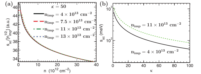
FIG. 7. (Color online) Self-consistent results. (a) s_{sc}/\sqrt{n_{imp}} (in units of \sqrt{10^{-13}} \text{ meV cm} ) as a function of carrier density for different values of n_{imp} with \kappa = 50 and d = 0.1 nm. (b) Potential fluctuation s_{sc} as a function of substrate dielectric constant \kappa . The solid lines are for n_{imp} = 4 \times 10^{13} \text{ cm}^{-2} and the dashed lines are for n_{imp} = 11.0 \times 10^{13} \text{ cm}^{-2} with d = 0.1 nm.
