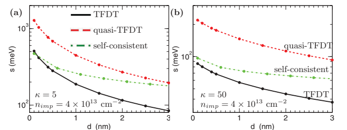
FIG. 8. (Color online) Comparison of three methods for the potential fluctuation s at the Dirac point versus the charged impurity distance d to the TI surface for n_{imp} = 4.0 \times 10^{13} \text{ cm}^{-2} . The solid, dashed, and dot-dashed lines correspond to the TFDT, quasi-TFDT, and the self-consistent methods, respectively. (a) The effective background dielectric constant \kappa = 5 . (b) The effective background dielectric constant \kappa = 50 .
