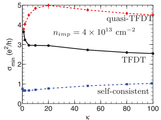
FIG. 12. (Color online) The minimum conductivity \sigma_{\text{min}} as a function background dielectric constant \kappa for n_{\text{imp}} = 4.0 \times 10^{13} \text{ cm}^{-2} , d = 0.1 nm. The dashed, solid, and dot-dashed lines denote the results obtained using the quasi-TFD, TFD-EMT, and the self-consistent method, respectively.
