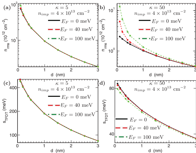
FIG. 6. (Color online) (a) and (b) n_{rms} at the Dirac point versus the distance d of the charged impurity to the TI surface calculated within TFDT for n_{imp} = 4.0 \times 10^{13} \text{ cm}^{-2} . The solid, dashed, and dot-dashed lines correspond to chemical potential E_F = 0, 40, and 100 meV, respectively. (c), (d) The corresponding s_{TFDT} results versus d . (a), (c) The effective background dielectric constant \kappa = 5 . (b), (d) The effective background dielectric constant \kappa = 50 .
