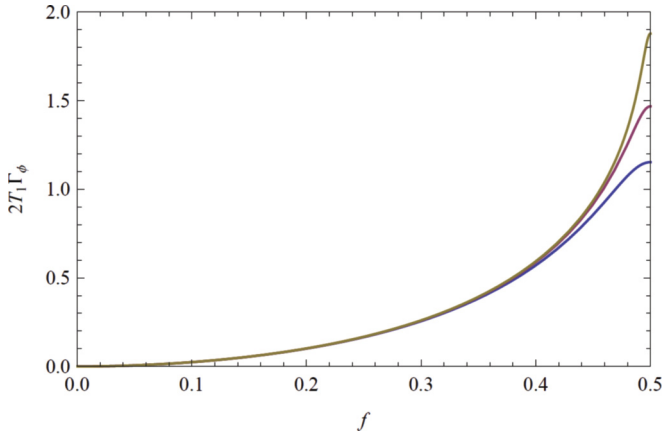
FIG. 2. (Color online) Normalized dephasing rate 2T_1\Gamma_\phi vs reduced flux f for (top to bottom) d = 0.02, 0.05, 0.1 . Other parameters are specified in the text after Eq. (56). The vanishing of \Gamma_\phi as f \rightarrow 0 is an artifact of the approximations used to obtain Eq. (56); a finite dephasing rate at any flux would be obtained by including a subleading contribution analogous to Eq. (45).
