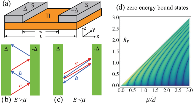
FIG. 1. (Color online) (a) Schematic of a Josephson junction on the surface of a topological insulator (TI). The two superconducting leads (S) have a phase difference \pi . \Delta is the superconducting gap, and w is the junction width (not to scale). (b) Specular Andreev reflection in the regime E > \mu . (c) Retroreflection for E < \mu . (d) Dark lines show the (k_y, \mu) values for the zero energy Andreev bound states for w = 10 \hbar v_F / \Delta and L \rightarrow \infty . k_y is in a unit of \Delta / \hbar v_F .
