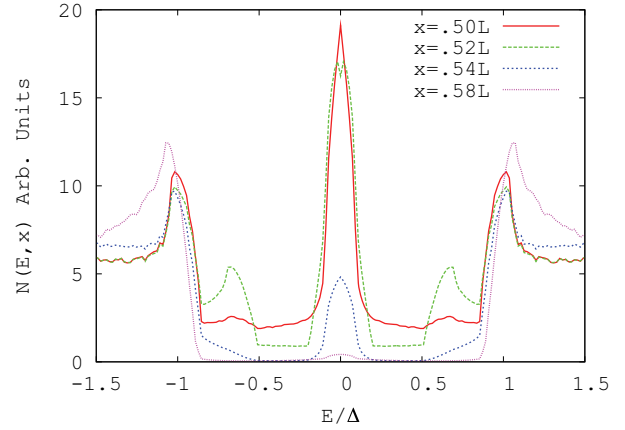
FIG. 2. (Color online) The local spectral function A_\uparrow(E, k_y, x) (upper panel) and local density of states N(E, x) (lower panel, red solid line) at the center of the junction, x = 0.5L . One sees “flat” Andreev bound states near zero energy for -k_F < k_y < k_F , and correspondingly a pronounced peak at zero energy in the LDOS in the lower panel. The lower panel also shows different LDOS away from the center, for x from 0.52L to 0.58L .
