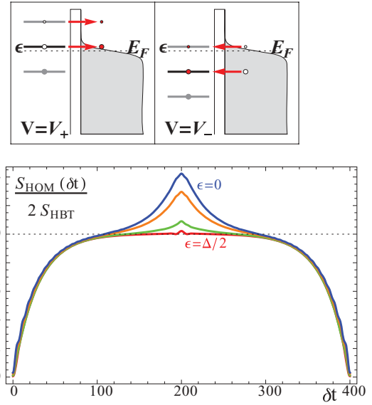
FIG. 3. (Color online) Upper panel: Electron (left) and hole (right) emission process, for a square voltage drive, for the two positions of the dot levels (values V_+ and V_- of the drive). The position of the dot levels is parametrized by \epsilon with respect to E_F . Bottom panel: HOM peak for electron-hole collision, for a square voltage drive, at different level positions \epsilon = 0.5, 0.4, 0.25 , and 0 (in units of \Delta ) from the smallest to the largest peak. T = 0.1\Delta in both panels.
