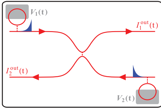
FIG. 1. (Color online) The device. Two chiral edge states meet at a quantum point contact. In each edge state a single electron source injects an electron when a time-dependent voltage V(t) is applied at the source. Cross correlations at the two outputs are measured as a function of the time difference between the electrons which are emitted by each source.
