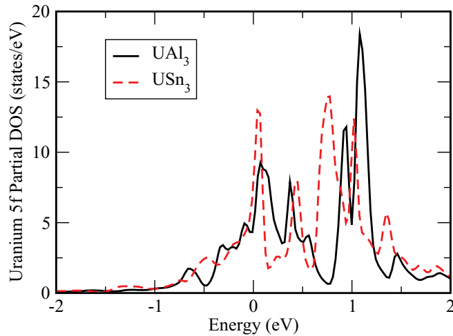
FIG. 2. (Color online) Uranium 5 f partial DOS calculated from the LAPW method for UAl 3 and USn 3 , in the magnetic unit cell, in the energy range (−2,2) eV. Note the narrower peak width near the Fermi energy ( E = 0 ) in USn 3 compared to UAl 3 .
