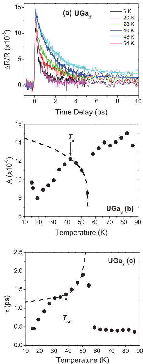
FIG. 5. (Color online) (a) Photoinduced change in reflectivity \Delta R/R versus pump-probe time delay at different temperatures of UGa 3 . Thick blue (cyan) curves denote one-exponential fits of data at T = 40 K (48 K). Temperature dependence of (b) amplitude and (c) relaxation time for UGa 3 obtained from one-exponential fits, with dashed lines in (b) and (c) being fits to the RT model from 40 K to T_N .
