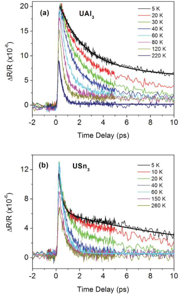
FIG. 1. (Color online) Transient reflection \Delta R/R versus pump-probe time delay at different temperatures for (a) \text{UAl}_3 and (b) \text{USn}_3 . Thick solid curves denote exponential fits of data, for \text{UAl}_3 (at 5 K and 220 K) and \text{USn}_3 (at 5 K and 60 K).
