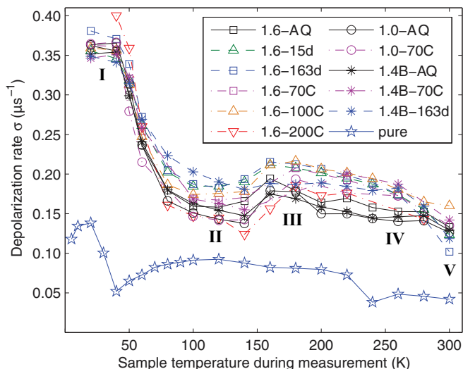
FIG. 3. (Color online) Muon depolarization rate in pure Al (99.99%) and Al-Mg-Si alloy conditions in Table I as a function of temperature. The fit errors are roughly as large as the markers.
