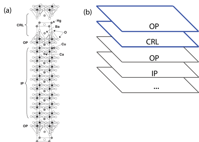
FIG. 2. (Color online) (a) The n -layer Hg cuprate consists of n - 2 inner planes (IP), two outer planes (OP), and a CRL. In this family, T_c exhibits no variation with n beyond n > 5 and is close to T_c(n = 1) [reproduced with permission from J. Phys. Soc. Jpn. 76 , 094711 (2007)]. (b) For sufficiently large n , the inner planes are undoped and the outermost plane exhibits superconductivity. The minimal description in this limit reduces to that of a bilayer consisting of an OP layer and a CRL as shown in (b).
