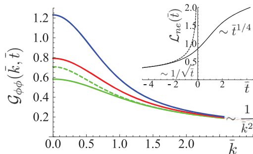
FIG. 5. (Color online) \mathcal{G}_{\phi\phi} for the linear TCP. The blue, red, and green solid lines are, respectively, at \bar{t} = 0.5, 0 , and -0.5 . The green dashed line is the correlator if the system were in equilibrium at \bar{t} = -0.5 . Inset: \mathcal{L}_{ne} vs \bar{t} (solid line) and \xi/l_0 (dashed line).
