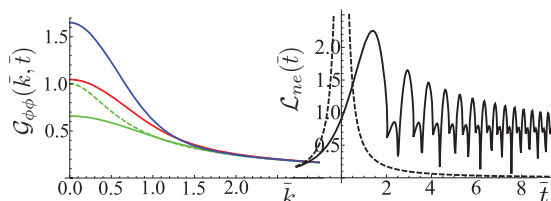
FIG. 7. (Color online) Left: \mathcal{G}_{\phi\phi} for the quadratic CCP. The blue, red, and green solid lines are, respectively, at \bar{t} = 0.5, 0, and -0.5 . The green dashed line is the correlator if the system were in equilibrium at \bar{t} = -0.5 . Right: \mathcal{L}_{\text{ne}} vs \bar{t} (solid line) and \xi/l_\rho (dashed line).
