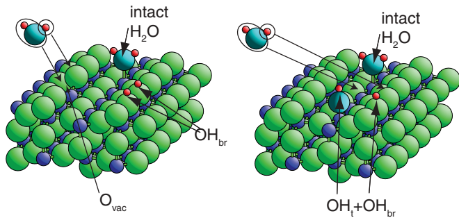
FIG. 1. (Color online) Schematic diagram of the interaction of molecular \text{H}_2\text{O} with \text{TiO}_2(110) on (left) a surface containing bridging oxygen vacancies, \text{O}_{\text{vac}} , to produce two bridging hydroxyl species, \text{OH}_{\text{br}} and (right) on a perfect surface to produce atop and bridging hydroxyl species, \text{OH}_t and \text{OH}_{\text{br}} . The diagrams show both of the component parts of a water molecule approaching the dissociation sites and the resulting pair of surface OH species produced. At low temperatures coadsorbed intact molecular water also occupies Ti-atop sites.
