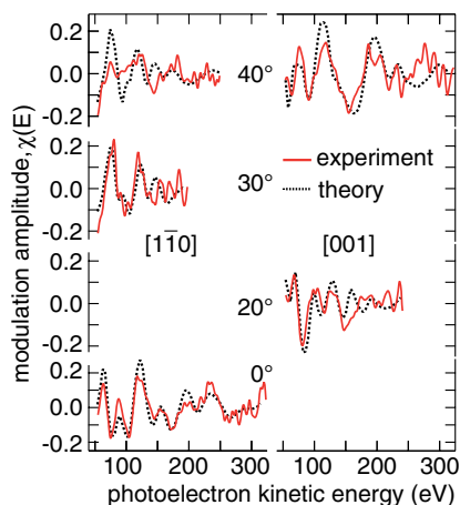
FIG. 2. (Color online) Comparison of the experimental O 1s (OH) PhD spectra with theoretical simulations for the best-fit structure discussed in the text.
