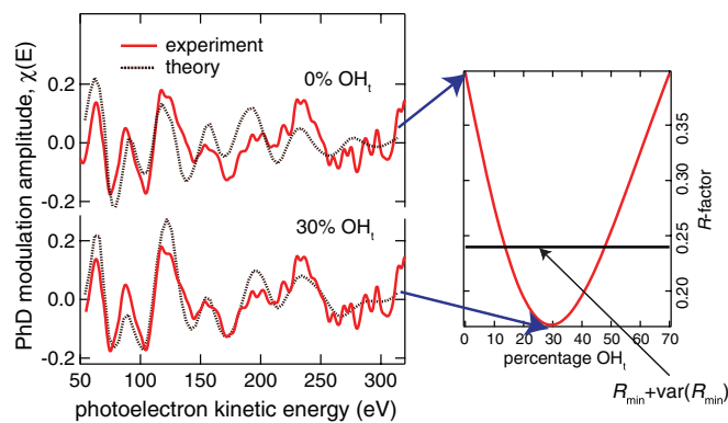
FIG. 3. (Color online) Dependence of the level of agreement between experiment and theory for the normal emission PhD spectrum as a function of the fractional occupation of OH t species. On the left are shown theory/experiment comparisons for 0% and 30% OH t occupation; on the right is shown the dependence of the R factor on this parameter.
