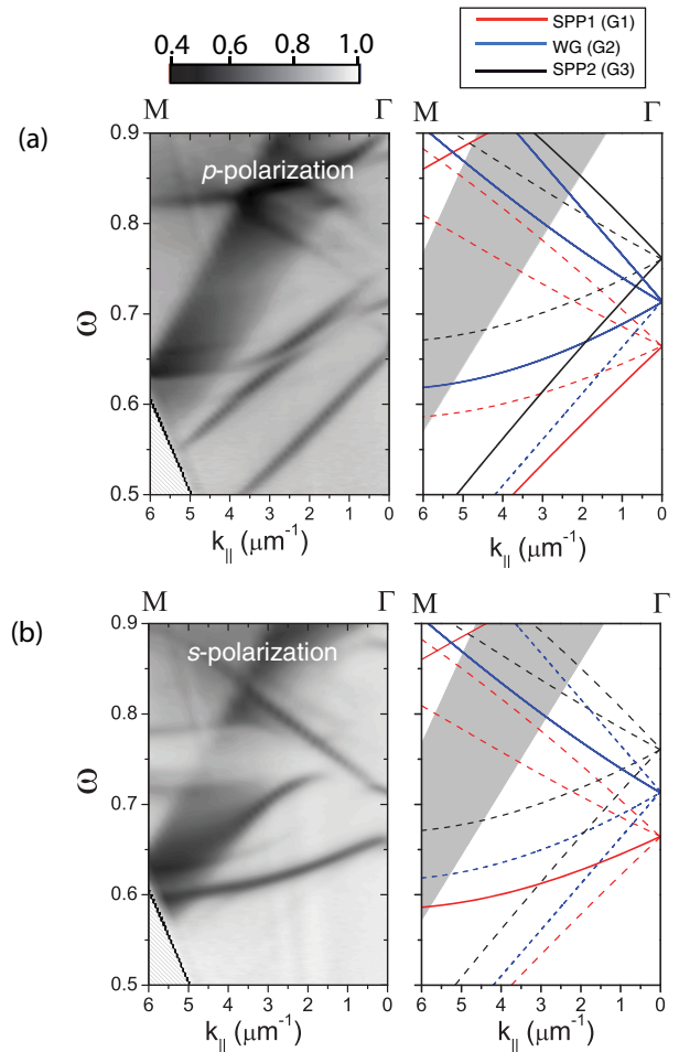
FIG. 5. (Color online) Angle-resolved reflectance for a monolayer of polystyrene spheres grown on a 60-nm silver film measured along the \Gamma\text{M} direction in reciprocal space for p - (a) and s - (b) polarized light. Right panels show dispersion relations calculated using an effective medium model (see text). Solid lines are highlighted branches of the calculated dispersion relation, which reproduce experimental data.
