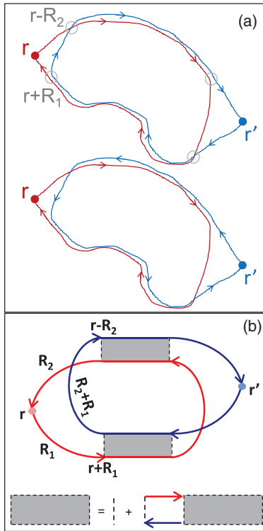
FIG. 1. (Color online) (a) Returning quasiparticle trajectories leading to the long-range correlations between the points \mathbf{r} and \mathbf{r}' . The trajectories are characterized by two pieces of long joint routes within which the diffusing particles move either in the same or in the opposite directions. (b) Two-diffuson diagram describing long-range part of the LDoS correlation function. Upper (lower) loop represents G^R(E, \mathbf{r}', \mathbf{r}') [ G^A(E, \mathbf{r}, \mathbf{r}) ] correspondingly. Shaded box represents diffuson. The two-cooperon contribution can be obtained by reversing arrows direction in one of the loops.
