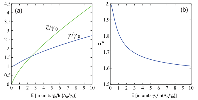
FIG. 4. (Color online) (a) The energy dependencies of the parameter \tilde{\epsilon} and the relaxation rate \gamma . (b) The energy dependence of the function F_d , which determines the LDoS correlation function in Eq. (38).
