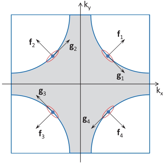
FIG. 3. (Color online) Schematic Fermi surface for a cuprate d -wave superconductor. \mathbf{f}_n and \mathbf{g}_n represent, respectively, the unity vectors parallel to the Fermi velocity \mathbf{v}_f and the “gap velocity” \mathbf{v}_g at the n th gap node. The ellipses illustrate the constant-energy surfaces near the nodes.
