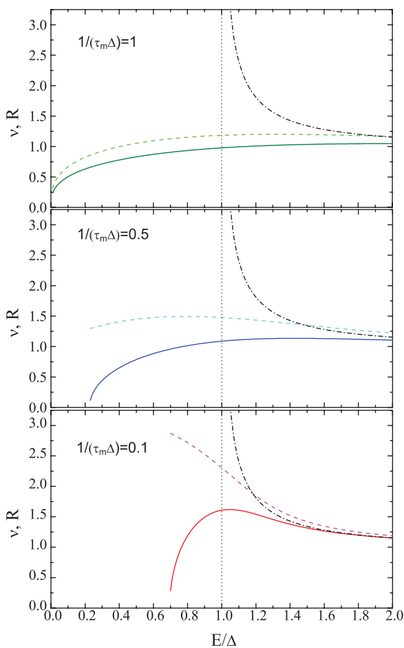
FIG. 2. (Color online) Examples of the energy dependences of the normalized average DoS \nu_{\text{ex}}^{(\text{sm})}(E)/(2\nu) , Eq. (25), (solid lines), and function |\mathcal{R}(E)| , Eq. (29), (dashed lines), which determines the long-range LDoS correlations for 1/(\tau \Delta) = 5 and different values of 1/(\tau_m \Delta) . Dash-dotted lines show for reference the BCS density of states.
