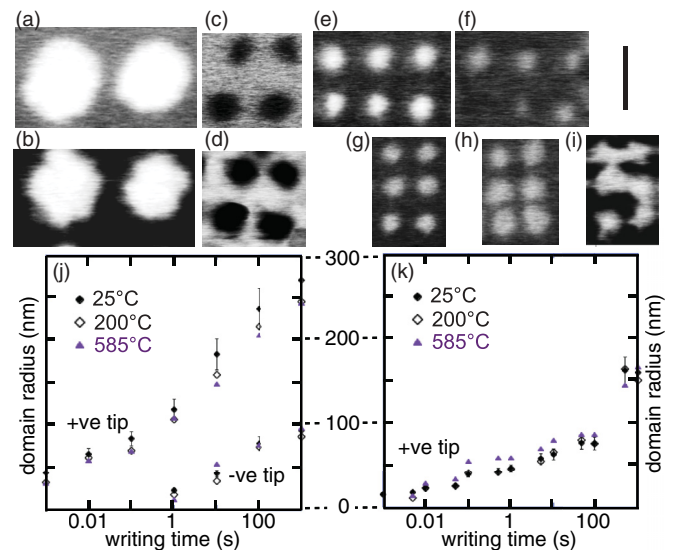
FIG. 4. PFM images of nanoscale ferroelectric domains written at ambient conditions in the 91-nm PZT film (P UP as grown) with (a) 1-s, +12-V, (c) 10-s, -10-V, (e) 1-ms, +12-V pulses, and in a 52-nm PZT film (P DOWN as grown) with (g) 100-ms, +12-V pulses. Domain evolution after thermal cycling [(f) and (h)] to 200°C and [(b), (d), and (i)] 585°C. Vertical bar = 250 nm. All images are shown to the same scale. The average domain size as a function of the writing time at ambient conditions, and after thermal cycling up to the indicated temperatures (j) for the 91-nm film and (k) for the 52-nm film.
