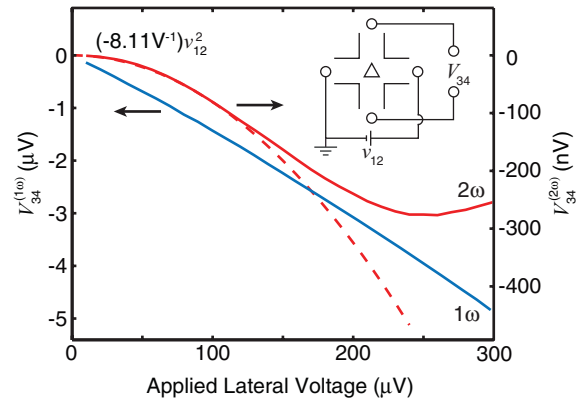
FIG. 3. (Color online) Main figure: First and second harmonic transverse responses, V_{34} , to a laterally applied 37 Hz voltage v_{12} . Also shown is a parabolic fit to the 2\omega curve at low voltages. Inset: Circuit schematic for the applied voltage measurement.
