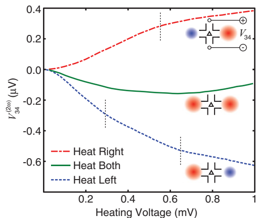
FIG. 4. (Color online) 2\omega transverse response due to heating both side channels simultaneously and individually. The vertical dotted lines indicate the approximate onsets of nonlinear regimes.
