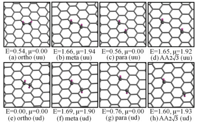
FIG. 2. (Color online) Models for the chemisorbed hydrogen dimers on the graphene plane. The (uu) in (a)–(d) indicate that two hydrogen adatoms are on the up side of the plane. The same dimer configurations with one hydrogen adatom on the up and the other one on the down side, as depicted with (ud), are shown in (e)–(h). The total energy differences (eV) are given with respect to the case of ortho(ud). Atomic symbols follow the same convention as in Fig. 1.
