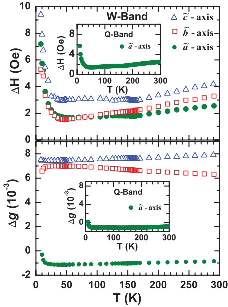
FIG. 7. (Color online) Temperature dependence of the W -band ESR linewidth and the g shift of (\text{TMTTF})_2\text{SbF}_6 along the three principal magnetic axes \tilde{a} , \tilde{b} , and \tilde{c} . The insets show the ESR linewidth and the g shift measured in the Q -band spectrometer along the \tilde{a} axis. The solid green dots correspond to the \tilde{a} axis, the open red squares to the \tilde{b} direction, and the open blue triangles to the \tilde{c} axis.
