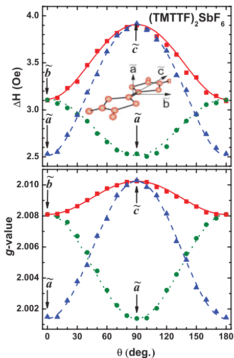
FIG. 2. (Color online) Angular dependence of the ESR linewidth \Delta H (HWHM) (top), and the g value (bottom) of (\text{TMTTF})_2\text{SbF}_6 at room temperature measured at X -band frequency when the static magnetic field B_0 is rotated within the \tilde{a}\tilde{b} plane (green circles), the \tilde{b}\tilde{c} plane (red squares), and the \tilde{a}\tilde{c} plane (blue triangles). The least-squares fits of the linewidth and the g value by Eqs. (1) and (2) are shown by the corresponding lines. The inset demonstrates the orientation of the different orthogonal directions within the TMTTF molecule. The \tilde{a} axis is normal to the plane, the \tilde{c} axis points in the long direction, and \tilde{b} points along the intermediate short direction.
