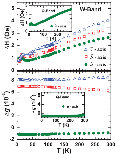
FIG. 8. (Color online) Temperature dependence of the W -band ESR linewidth and the g shift of (\text{TMTTF})_2\text{AsF}_6 along the three axes \tilde{a} , \tilde{b} , and \tilde{c} . The Q -band ESR linewidth and the g shift ( \tilde{a} axis) are displayed in the insets, respectively.
