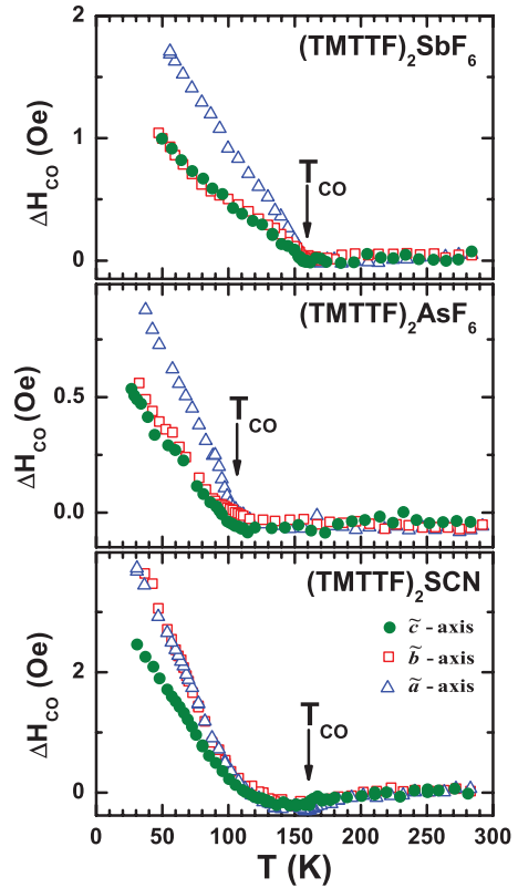
FIG. 9. (Color online) Contributions to the ESR linewidth due to CO for the salts (\text{TMTTF})_2X ( X = \text{SbF}_6, \text{AsF}_6, \text{and SCN} ) along the three main axes. Note the different scales of \Delta H_{\text{CO}} . The excess linewidth \Delta H_{\text{CO}}(T) is given by \Delta H(T) - \Delta H_{\text{background}}(T) and explained in the text. Note, the data are shown for temperatures well above the magnetic ordering and spin Peierls transitions that occur for T < 20 K.
