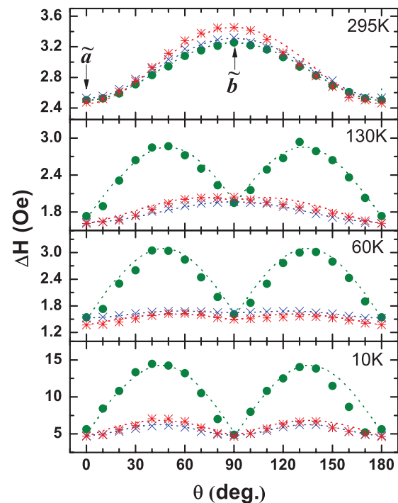
FIG. 10. (Color online) Angular dependence of the ESR linewidth within the \tilde{a}\tilde{b} plane of (\text{TMTTF})_2\text{SbF}_6 measured at different temperatures above and below the CO transition T_{CO} = 156 K using X-band (blue crosses), Q -band (red stars), and W -band (green dots) spectrometers. The lines represent fits of the linewidth using Eqs. (4) and (5) (see text for more details).
