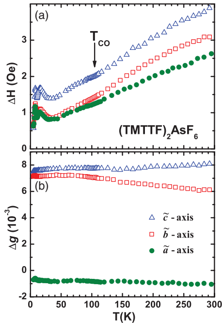
FIG. 5. (Color online) Temperature dependence of (a) the ESR linewidth \Delta H and (b) the g shift \Delta g(T) = g(T) - 2.002319 for (\text{TMTTF})_2\text{AsF}_6 measured by X -band spectroscopy along the three directions \tilde{a} (green dots), \tilde{b} (open red squares), and \tilde{c} (blue triangles).
