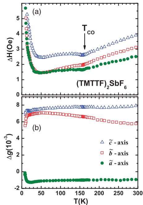
FIG. 4. (Color online) Temperature dependence of (a) the linewidth \Delta H , and (b) the change in the g value for (\text{TMTTF})_2\text{SbF}_6 measured by X -band ESR along the three crystal orientations. The green solid dots correspond to the \tilde{a} axis, the open red squares indicate the \tilde{b} direction, and the blue triangles are measured along the \tilde{c} direction.
