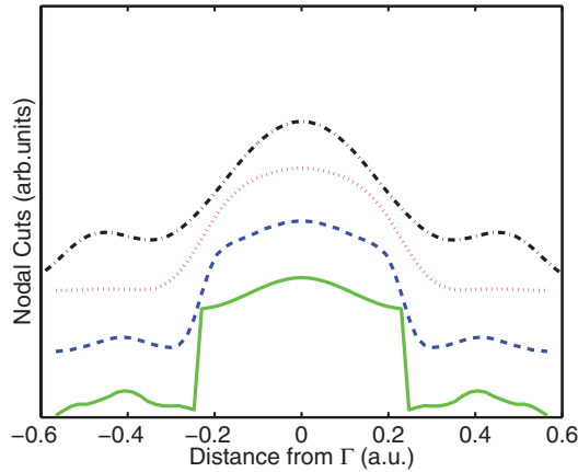
FIG. 8. (Color online) Cuts of the distributions in Fig. 7 along the nodal direction. The amplitudes of theory and experiment are compared on the same scale. Curves are offset with respect to one another for clarity. From the bottom to the top, the first curve is the nonconvoluted theory, the second is the convoluted theory with a resolution 0.07 a.u., the third is the convoluted theory with a resolution 0.13 a.u., and the fourth curve is the experimental data.
