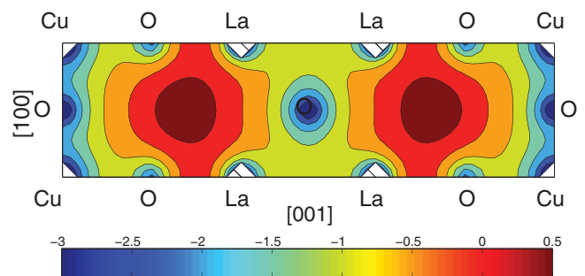
FIG. 5. (Color online) Positron density for LSCO in the (010) plane. The positron wave function is normalized in the LSCO unit cell and a logarithmic density scale (with integer numbers as units) is used in order to enhance regions with low positron density. The atomic positions (La, Cu, O) set the scale for the x and y axes.
