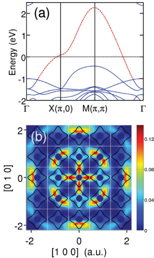
FIG. 1. (Color online) (a) Band structure of LSCO near the Fermi level. The \text{CuO}_2 band is shown as a red dotted line. (b) Calculated \rho_{x^2-y^2}^{2d}(p_x, p_y) is shown together with the FS sections at (k_z = 0) for the doping level x = 0.3 . The color scale is in units of \rho^{2d}(0,0) . The grid represents Brillouin zones with a size of 2\pi/a , where a is the lattice constant.
