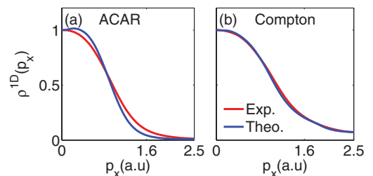
FIG. 2. (Color online) Theoretical and experimental profiles \rho^{1d}(p_x) for (a) ACAR and (b) Compton scattering along the [100] direction. All spectra are normalized to \rho^{1d}(0) .
