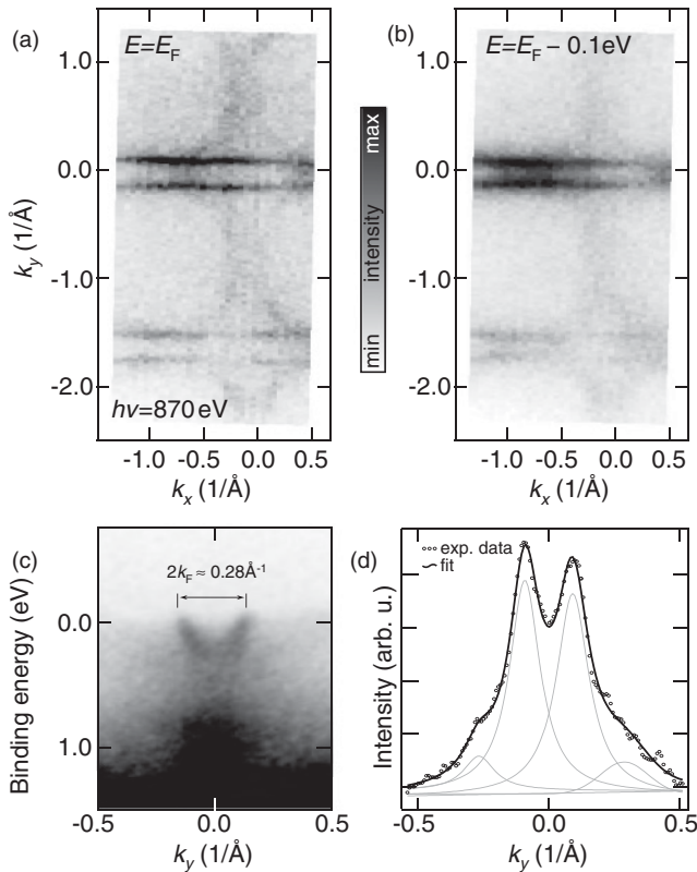
FIG. 5. (a), (b) Momentum intensity distribution at the Fermi level and at 0.1 eV below the FL for \text{YBa}_2\text{Cu}_3\text{O}_{6.4} . (c) Energy-momentum cut along the \text{Y}-\Gamma-\text{Y} direction. (d) MDC centered at binding energy of 170 meV and integrated over \pm 60 meV wide window. In the MDC fit the inner two peaks correspond to the subsurface chains, while the outer two are due to the remnant spectral weight of the heavily disordered surface chains.
