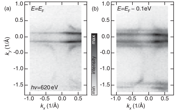
FIG. 3. (a), (b) Momentum intensity distribution at the Fermi level and at 0.1 eV below the FL for YBa 2 Cu 3 O 6.6 . The right image reveals another 1D band, which contributes practically no spectral weight at the Fermi level. Spectra measured with p -polarized light and energy resolution of 90 meV.
