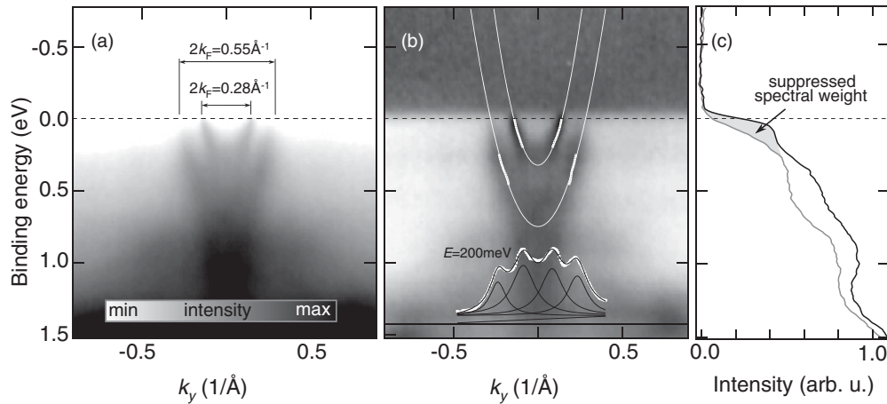
FIG. 4. (a) Energy-momentum cut along the Y- \Gamma -Y direction demonstrating two types of chain bands in YBa 2 Cu 3 O 6.6 . (b) The same as previous, but each MDC in the image has been normalized to 1. The small square symbols denote the peak positions obtained in a four-Lorentzian MDC fit. The inset shows typical fit for the MDC at E_B = 200 meV. The obtained experimental dispersions are fit to parabolic bands (solid white lines). (c) k_F EDC's for the inner chain band (black line) and outer chain band (gray line). Polarization and resolution are the same as in Fig. 3.
