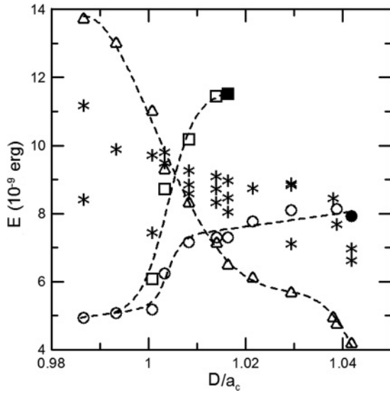
FIG. 6. Calculated energies of the magnetic configurations for different ratios between magnetic disk diameter ( D ) and lattice constant ( a_c = 300 nm). Triangles denote the energy of the system with the dots in the single-domain states. Squares denote the energies of the frustrated lattices of the magnetic vortices for the configuration when all interdot contacts are antiferromagnetically aligned. The circles are for the lattice of the magnetic vortices configuration when 1/3 of the interdot contacts are antiferromagnetically aligned while 2/3 are aligned ferromagnetically. The solid square and the solid circle are for the maximum D/a_c value when the corresponding vortex configurations remain stable. Stars denote the energies of different mixed configurations. The dashed lines are guides for the eyes.
