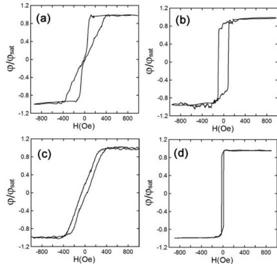
FIG. 2. In-plane magnetization curves of the lattices of the Co nanocaps measured by the magneto-optic Kerr rotation. (a) Hysteresis loop of the 30-nm Co film deposited on the top of the PMMA colloidal crystal (the particle diameter is 340 nm). The loop corresponds to the vortex distribution of the magnetization in the caps. (b) Hysteresis loop of the 30-nm film deposited on the top of the PMMA colloidal crystal (the particle diameter is 120 nm). The loop corresponds to the single-domain distribution of the magnetization in caps. (c) Hysteresis loop of the 60-nm film deposited on the top of PMMA colloidal crystal (particle diameter 290 nm). The loop corresponds to the mixed states of the magnetization distribution in the system. (d) Hysteresis loop of the flat control Co film.
