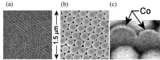
FIG. 1. (a),(b) SE images of the 30 nm Co film on the top of the colloidal crystals with the period 120 and 370 nm correspondingly. (c) Microphotography of the particles cross-section made by focused \text{Ga}^+ ion beam. The image observed with backscattered electrons ( E = 3 kV), the Co coverage is visible as bright layer.
