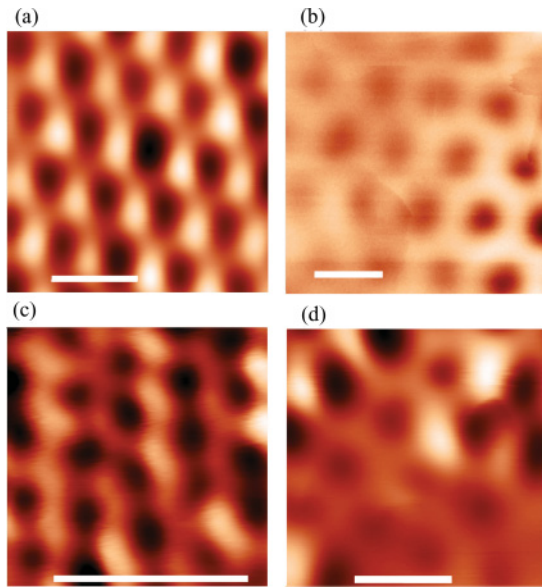
FIG. 3. (Color online) Experimental MFM images of the lattices of the Co nanocaps in different magnetic states at zero magnetic field. The length of the scale bar is equal to 400 nm. (a) MFM image of the lattice of the Co nanocaps (the particle diameter is 290 nm; Co thickness is 30 nm) at 200 Oe after magnetizing to the saturation at 1000 Oe. (b) The lattice of the magnetic vortices. (c) The lattice of single-domain states magnetized uniformly in the remanent state at zero magnetic field (the particle diameter is 120 nm; Co thickness is 30 nm). (d) The mixed distribution of the magnetization; both vortices and single-domain states are visible (the particle diameter is 290 nm; Co thickness is 60 nm). The particles with single-domain distribution produces two magnetic poles; the particles within vortex state produces less signal with centrally symmetric contrast.
